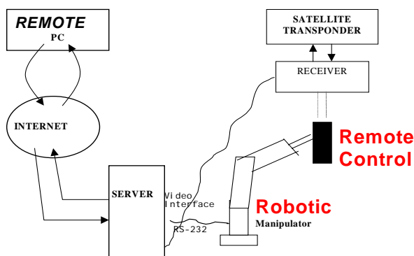
Figure 7: System Schematics
