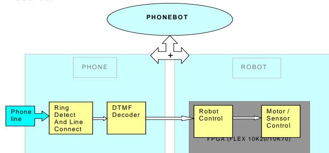
Figure 2: PHONEBOT – Basic Block Diagram
