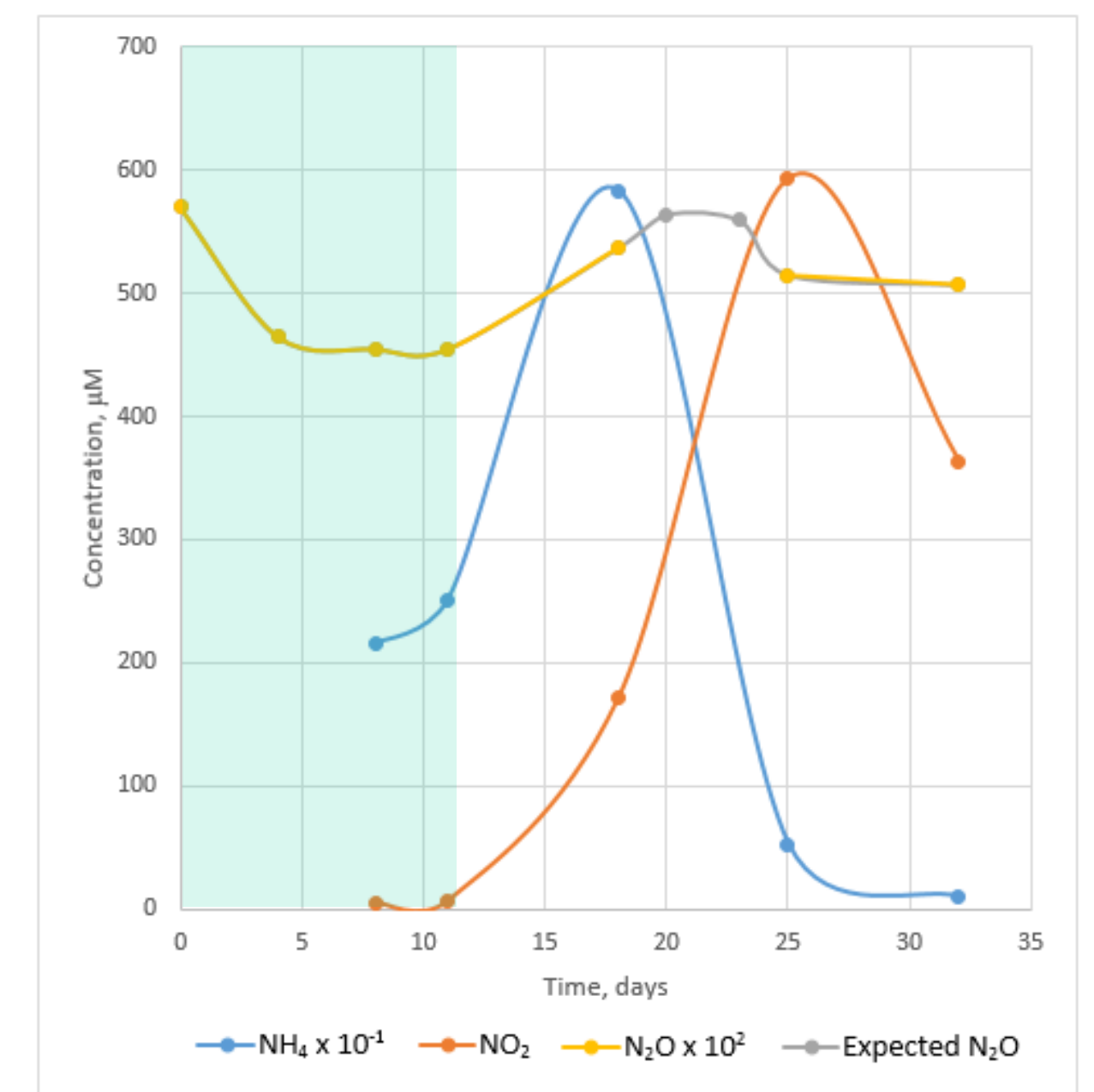
Figure 4. Shows the measurements of nitrogen species over time in beakers containing sediment saturated with biodeposits at 25°C. The shaded region denotes dark conditions. A calculated "expected N 2 O" has been added to extrapolate the measured data ( R^2: 0.875 , p < 0.0001 ).
