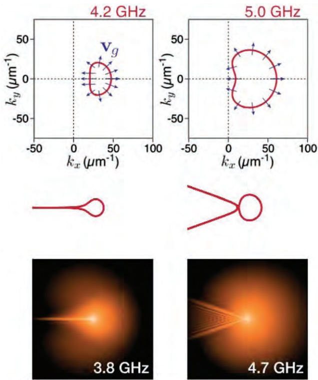
Figure 32. Isofrequency curves and the resulting focusing pattern for a thin ferromagnetic film influenced by iDMI. There is a magnetic field (vertically) parallel to the xy plane. The figures in the top panel show the isofrequency curves and the bottom sets of panels present the focusing patterns calculated analytically and numerically. Reprinted (figure) with permission from [200], Copyright (2016) by the American Physical Society.
