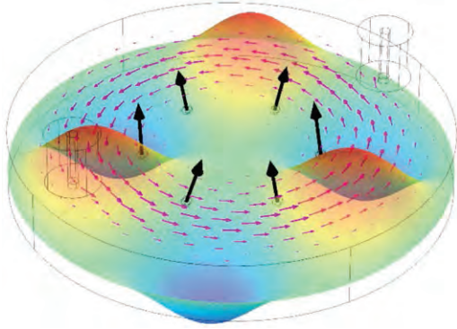
Figure 36. Numerical simulation of six magnetic spheres on a circle inside a disk-shaped microwave cavity fed by attached ports. At resonance, the magnetizations (black arrows) precess coherently in the presence of a unidirectional photon current as illustrated by the Poynting vector field (magenta arrows). The colored background is the electric field component in the perpendicular direction. We interpret this system as a chiral magnonic benzene molecule (Yu et al 2020, Phys. Rev. B 102 , 064416).
