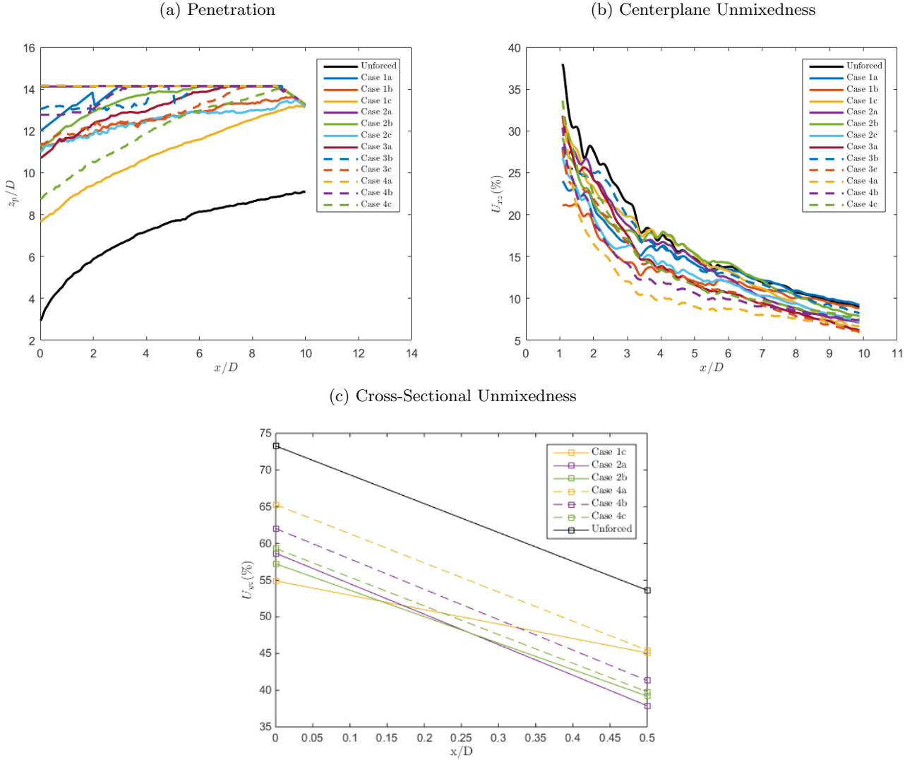
FIG. 11. (a) Mean centerline vertical jet penetration, z_p/D , (b) instantaneous quantifications of the downstream evolution of centerplane unmixedness, U_{xz} , and (c) instantaneous valuations of cross-sectional unmixedness at downstream locations of x/D = 0.0 and 0.5 , U_{yz} , of the JICF at J = 10 for various double-pulse forcing cases, averaged over 500 instantaneous images.
