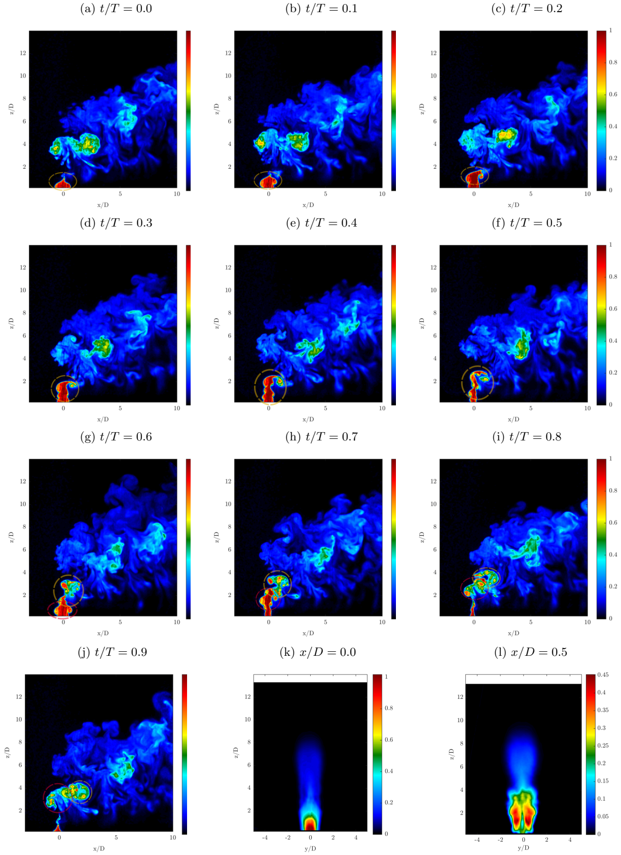
FIG. 7. Representative PLIF images of the double-pulse forced AU jet at J = 7 , for forcing case 1c where (a-j) depict the instantaneous centerplane phase progression at every tenth of a the forcing period, and (k-l) are mean cross-sectional slices of the jet at x/D = 0.0 and x/D = 0.5 , respectively. Yellow and red dashed circles represent slow and quick pulse structures, respectively.
