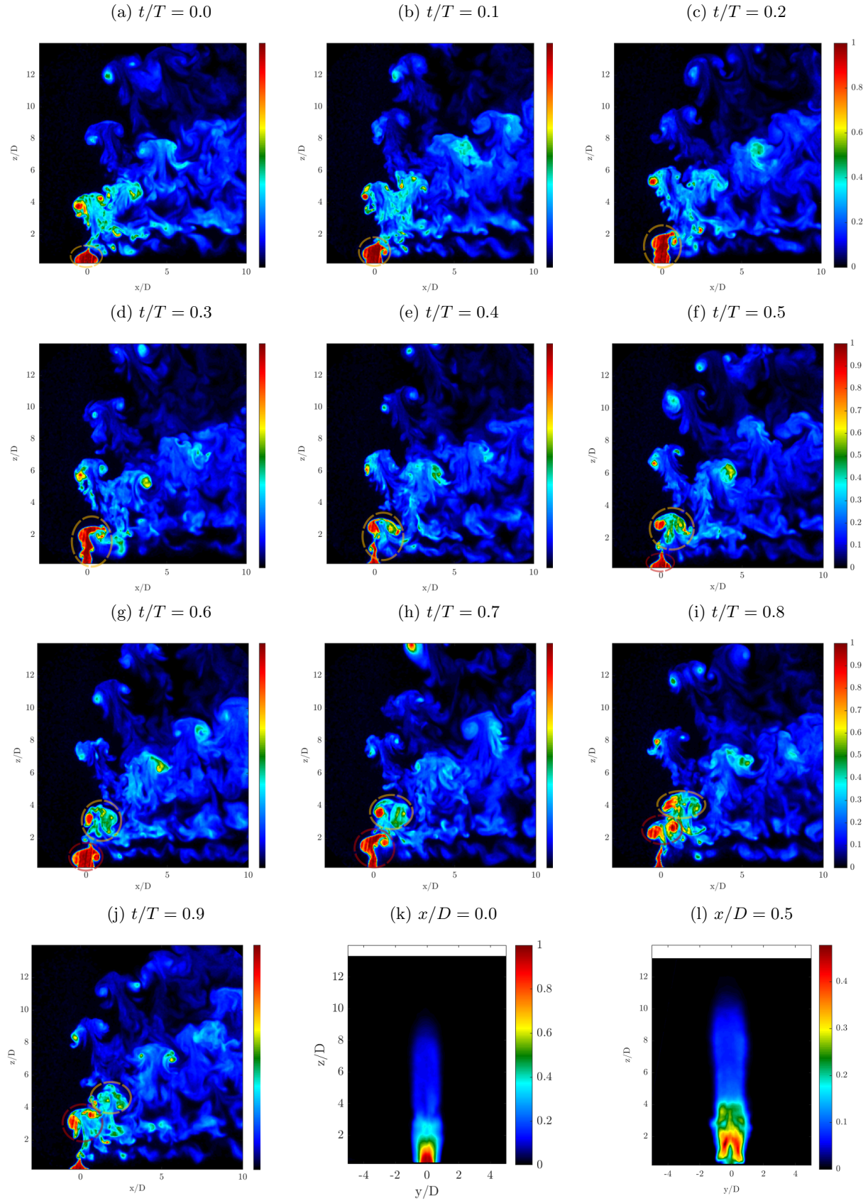
FIG. 8. Representative PLIF images of the double-pulse forced AU jet at J = 7 , for forcing case 2a where (a-j) depict the instantaneous centerplane phase progression at every tenth of a the forcing period, and (k-l) are mean cross-sectional slices of the jet at x/D = 0.0 and x/D = 0.5 , respectively. Yellow and red dashed circles represent slow and quick pulse structures, respectively.
