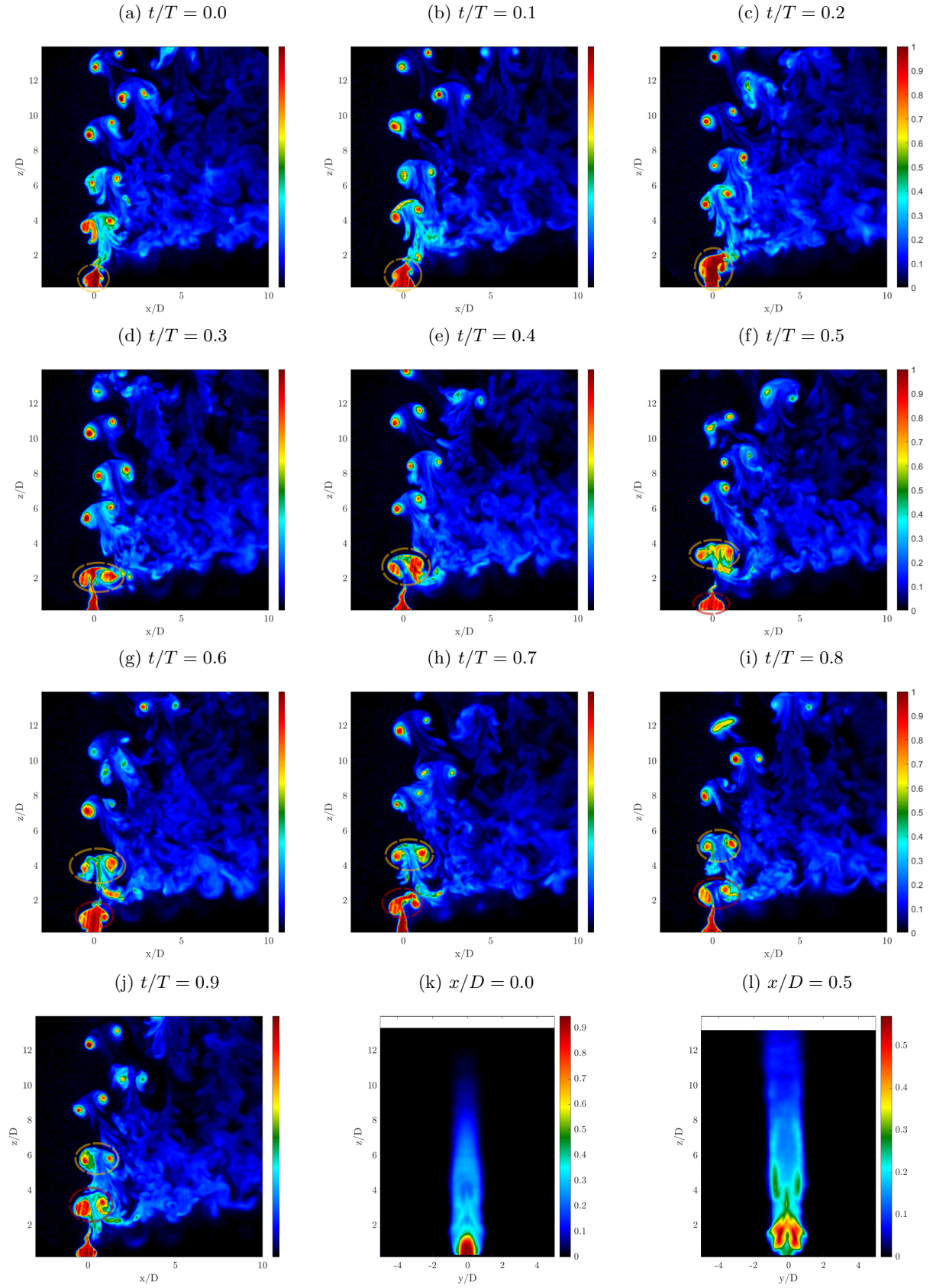
FIG. 9. Representative PLIF images of the double-pulse forced CU jet at J = 10 , for forcing case 4a where (a-j) depict the instantaneous centerplane phase progression at every tenth of a the forcing period, and (k-l) are mean cross-sectional slices of the jet at x/D = 0.0 and x/D = 0.5 , respectively. Yellow and red dashed circles represent slow and quick pulse structures, respectively.
