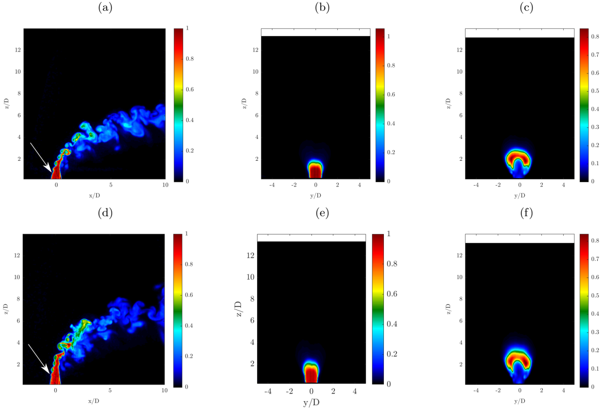
FIG. 6. Representative PLIF images of the unforced JICF at J = 7 ((a)-(c)) and at J = 10 ((d)-(f)), where (a,d) depict the instantaneous centerplane of the jet, and (b) and (e), and (c) and (f) are mean cross-sectional slices of the jet at x/D = 0.0 and x/D = 0.5 , respectively.
