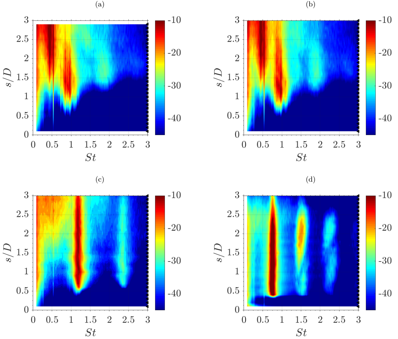
FIG. 4. Power spectra of the upstream shear layer instabilities for the equidensity large ( D = 7.59 \text{ mm} ) flush nozzle-injected JICF with acetone mole fraction of \psi = 0.218 , jet Reynolds number of Re_j = 1800 , and jet velocity of U_j = 3.31 \text{ m/s} at momentum flux ratios of (a) J = 15 with a fundamental frequency of f_0 \approx 410 \text{ Hz} , (b) J = 10 with f_0 \approx 420 \text{ Hz} , (c) J = 7 with f_0 \approx 540 \text{ Hz} , and (d) J = 3 with f_0 \approx 340 \text{ Hz} .
