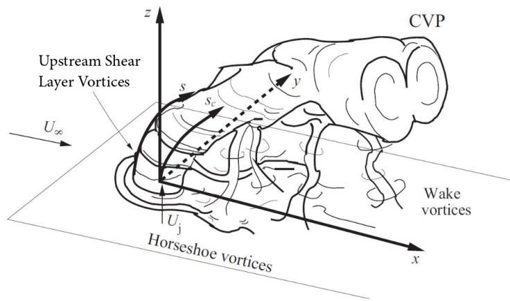
FIG. 1. Schematic of a flush round jet with mean velocity U_j injected normally into crossflow of freestream velocity U_\infty , with representative depictions of the relevant vortical structures. Appropriate coordinate axes x, y, z , jet shear layer trajectory s , and jet centerline trajectory s_c are also shown. Adapted from [13].
