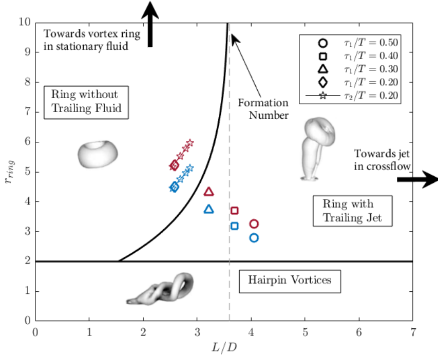
FIG. 5. Regime map of types of vortex rings formed based on the stroke ratio and ring velocity, with boundaries based on DNS of isolated vortex rings in crossflow ([44]). The L/D and r_{ring} values for different temporal pulse widths in the present experiments are shown for cases with J = 7 (blue) and J = 10 (red).
