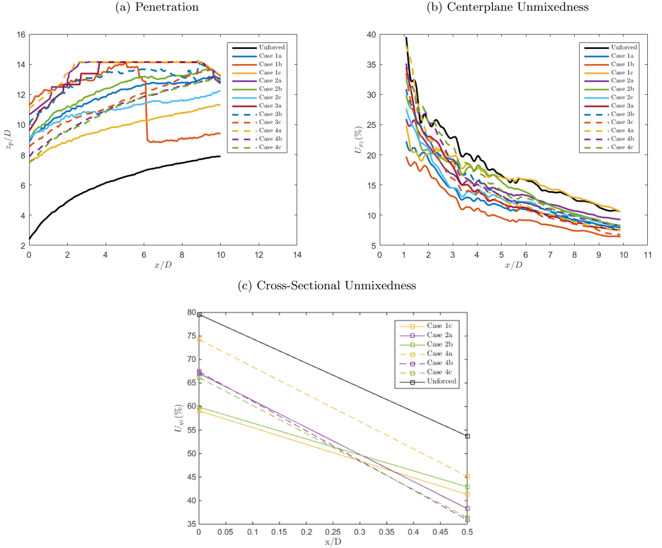
FIG. 10. (a) Mean centerline vertical jet penetration, z_p/D , (b) instantaneous quantifications of the downstream evolution of centerplane unmixedness, U_{xz} , and (c) instantaneous valuations of cross-sectional unmixedness downstream locations of x/D = 0.0 and 0.5 , U_{yz} , of the JICF at J = 7 for various double-pulse forcing cases, averaged over 500 instantaneous images.
