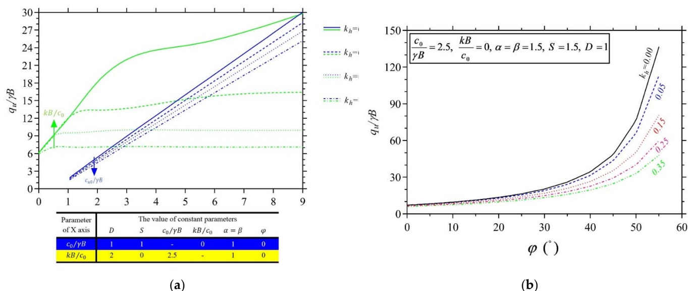
Figure 4. Parametric analysis: effects on the bearing capacity Q = q_u/\gamma B under different values of the seismic acceleration coefficient k_h , of: (a) the dimensionless soil parameters c_0/\gamma B (blue plots) and kB/c_0 (yellow plots); (b) internal friction angle \varphi .
