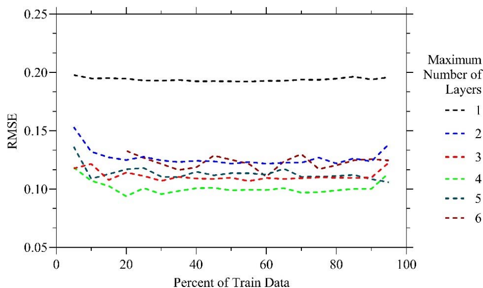
Figure 10. GMDH: dependence of the RMSE at the end of training on the maximum number of layers in the ANN, and on data proportioning.
