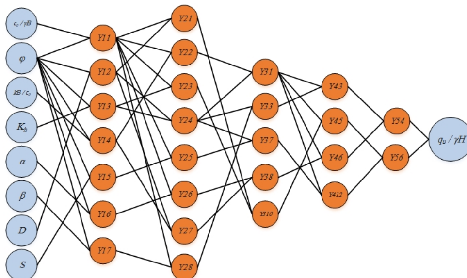
Figure A1. Architecture of the adopted GMDH model.
