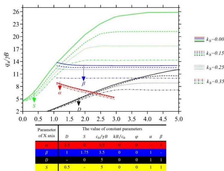
Figure 5. Parametric analysis: effects on the bearing capacity Q = q_u/\gamma B under different values of the seismic acceleration coefficient k_h , of the dimensionless void parameters \alpha (red plots), \beta (blue plots), S (green plots), and D (black plots).
