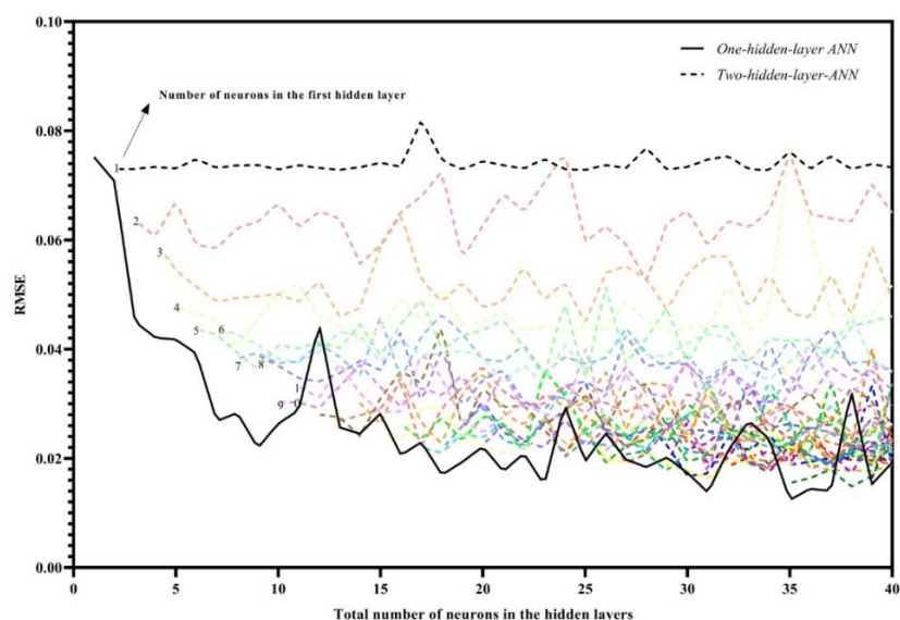
Figure 6. MLP: dependence of the RMSE at the end of training on the total number of neurons in the ANN, featuring either one or two hidden layers.
