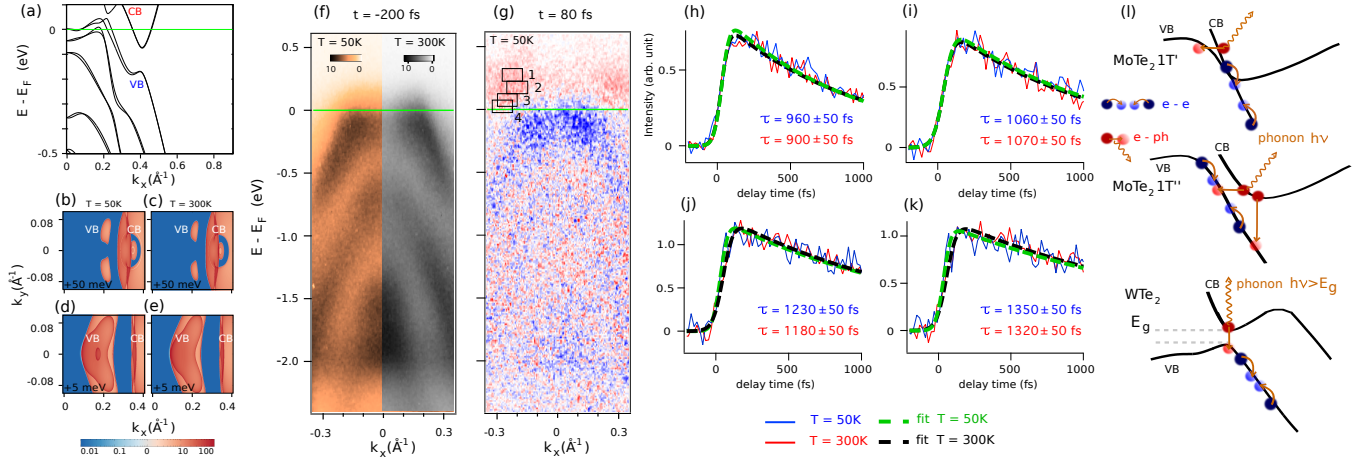
FIG. 3: (a) Band structure of WTe 2 along \Gamma X calculated for the low-temperature crystal lattice parameters. (b - e) Calculated k -resolved bulk density of states, projected on the [001] surface BZ, at two different binding energies for the crystal structure at low and high temperatures. Unlike the case of MoTe 2 the CB and VB are always well separated in momentum and energy. (f) Band structure along \Gamma X for WTe 2 measured at 50 K (left) and at 300 K (right) with 17.5 eV HHG photons. (g) The difference between ARPES images acquired 80 fs after and 200 fs before the arrival of a 2 eV optical excitation with fluence \sim 0.3 \text{ mJ/cm}^2 . (h - k) Comparisons of the dynamics in regions 1 - 4 at low (blue) and high (red) temperature. A fit to the traces (dashed green and black lines) yields quantitative estimations of the characteristic relaxation time, \tau , which is three times larger than the gapped 1T'' MoTe 2 . (l) Close-up on the calculated band structures of 1T' MoTe 2 , 1T'' MoTe 2 and WTe 2 in the region of the WPs. The possible electron – electron and electron – phonon scattering events are shown schematically.
