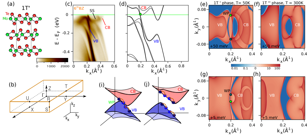
FIG. 1: Crystal structure (a) and three-dimensional Brillouin zone (b) of 1T' MoTe 2 [16]. (c, d) Experimental and calculated band dispersion of 1T' MoTe 2 along the \Gamma X high-symmetry direction. (e - h) Calculated k -resolved bulk density of states, projected on the [001] surface BZ, for the low- (e, g) and high- (f, h) temperature phases of MoTe 2 , at two different binding energies. The presence of two pairs of WPs is revealed in the 1T' phase, at 50 meV (e) and 5 meV (g), respectively. In the centrosymmetric 1T'' phase, the WPs vanish and the VB and the CB are well separated in momentum and in energy, as shown in the the CEMs at 50 meV (f) and 5 meV (h). (i, j) The cartoon shows that electron - electron interaction can mediate the scattering between CB and VB along the Weyl cone in the WSM phase (i). Interband scattering requires momentum and energy exchange in the presence of the gap (j).
