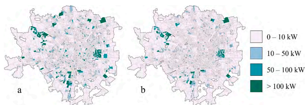
Figure 13. Maps of Census Units' characterization by hourly district heating consumption for space heating in a winter day at 9 a.m. (a) and 10 p.m. (b) in the city of Milan.
