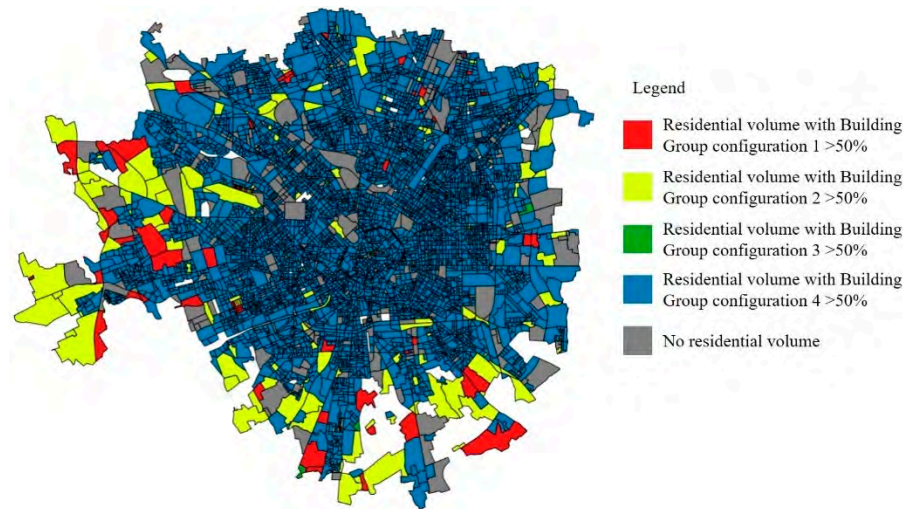
Figure 5. Maps of Census Units' characterization by prevailing Typical Thermal Zone in the city of Milan.
