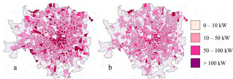
Figure 14. Maps of Census Units' characterization by hourly electricity consumption for space cooling, equipment, and lighting in a summer day at 9 a.m. (a) and 10 p.m. (b) in the city of Milan.
