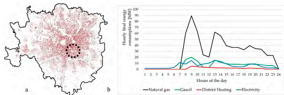
Figure 15. Selected mixed-use district in Milan (a) and related hourly-based energy consumption profiles for space heating, equipment, and artificial lighting in a winter day (b).
