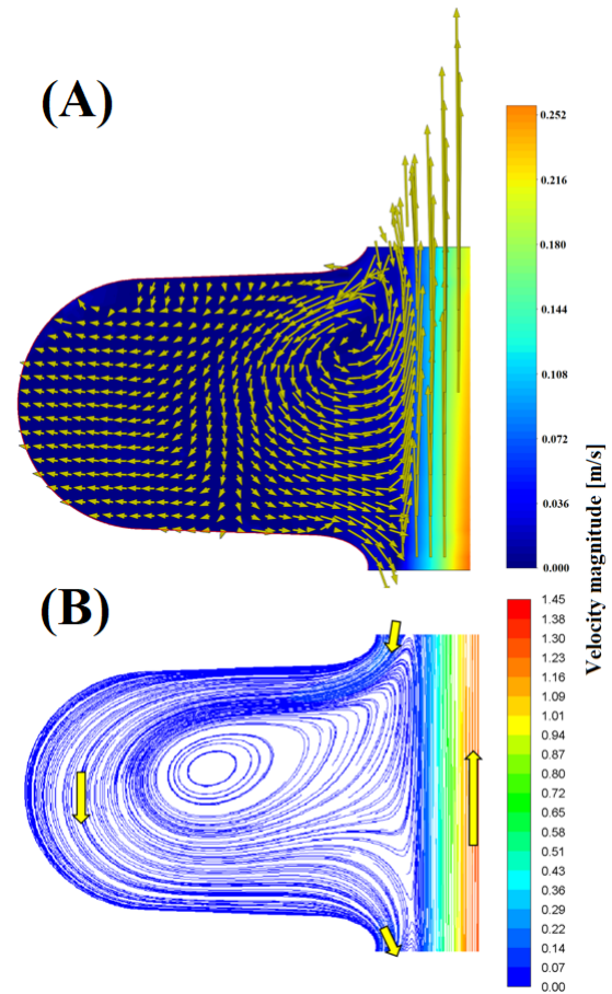
Figure 3: (A) PIV experimental results and (B) CFD simulations results.
