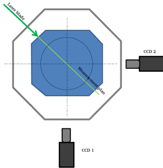
Figure 1: Schematisation of our PIV experimental set up.
