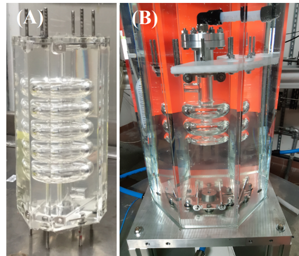
Figure 2: (A) Phantom model. (B) Experimental set up with phantom inside the aquarium filled with W-G mixture.
