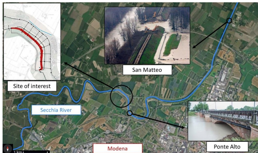
Fig. 1: Secchia river north to Modena city: locations of the breach failure in S. Matteo (2014) and of the site of the reprofiling intervention (2018) upstream to Ponte Alto [courtesy of Civil Protection Department, Italy].
