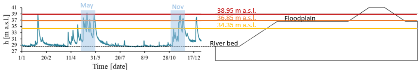
Fig. 4: River Secchia water levels in 2019 simulated in the analyses and schematization of the geometry of the case study (the horizontal scale is not respected). The hydrometric thresholds 1, 2 and 3 are represented respectively in yellow, orange and red.
