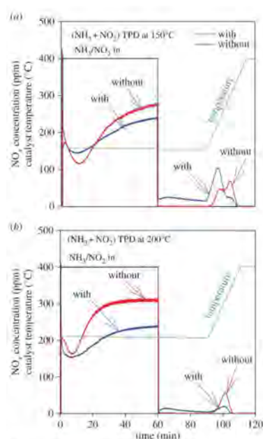
Figure 13. \text{NO}_x adsorption and desorption during (\text{NH}_3 and \text{NO}_2) TPD ‘with/without’ soot at (a) 150 and (b) 200 °C conducted over a DPF coated with SCR zeolite catalyst. Adsorption feed: 400 ppm \text{NH}_3 and 400 ppm of \text{NO}_2 , 8% \text{O}_2 , and 5% \text{H}_2\text{O} for 1 h, followed by exposing the catalyst to 5% \text{H}_2\text{O} in Ar for 30 min; thereafter, the temperature was increased to 400 °C. Reprinted with permission from ref. [87]. Copyright 2016 Royal Society of Chemistry.
