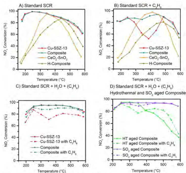
Figure 10. Comparison of the \text{NO}_x SCR activity of the investigated catalysts: Standard SCR (A), Standard SCR with HC (B), Standard SCR with \text{H}_2\text{O} and \text{C}_3\text{H}_6 added (C), and after ageing and \text{SO}_2 poisoning (D). Reprinted with permission from ref. [70]. Copyright 2021 Elsevier.
