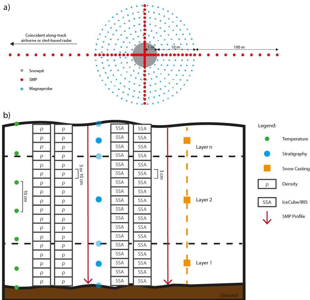
540 Figure 11: Optimal measurement configurations for evaluation of snow properties in sensor footprints.
