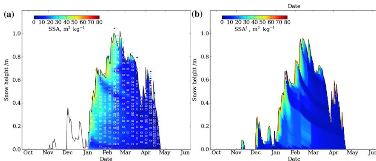
Figure 12: Observed and interpolated SSA observations (a) and SSA simulations (b). From Morin et al. (2013). The small white marks are the observations.
