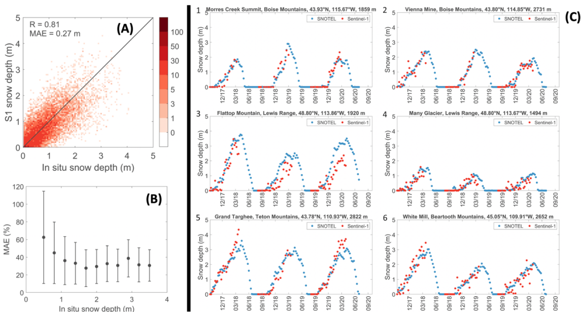
965 Figure 16: Snow depth retrieval from Sentinel-1, 2017-2020 in Idaho, Montana, and Wyoming. (a) Density plot of weekly 300-m resolution S1 snow depth retrievals, and coincident SNOTEL observations from 203 sites. (b) The corresponding mean and standard deviation of the absolute error between S1 retrievals and in situ measurements, stratified by the measured snow depth. (c) Time series comparison between snow depth from S1 and SNOTEL in situ measurements at six locations for three winter seasons. Note that the analysis includes snow-free conditions but excludes wet snow conditions as detected with the S1 algorithm (Lievens et al., 970 submitted).
