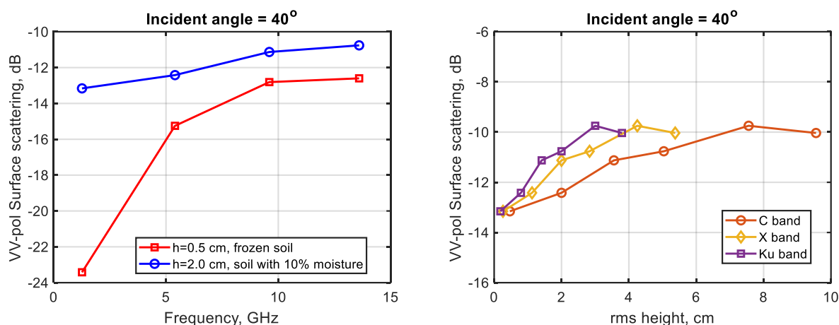
290 Figure 5: (a) Backscattering at VV-polarization as a function of frequency: red curve is results with frozen soil (permittivity 4+1i) and rms height 0.5 cm and blue curve is results with soil of 10% moisture and rms height 2 cm. (b) Backscattering at VV-polarization as a function of rms height with soil of 10% moisture at C-, X-, and Ku-band.
