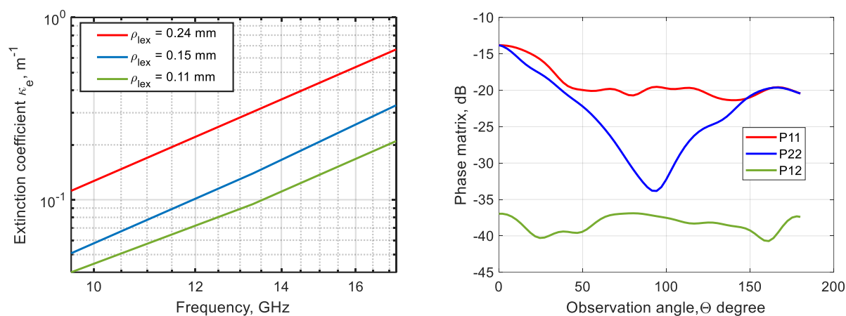
225 Figure 3: (a) Frequency dependence of the extinction coefficient from X- to Ku-band and (b) phase matrices at 13.3 GHz for different values of microstructure correlation length \rho_{lex} . Snow parameters are volume fraction f_v = 0.20 , aggregation parameter b = 1.2 , and correlation length 0.15 mm. P11 and P22 are co-polarized phase matrix elements and P12 is a cross-polarized phase matrix element.
