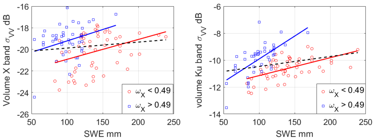
860 Figure 14: volume scattering of the Canada SnowSAR data as a function of SWE based on the retrieved scattering albedo \omega_X at (a, left) X-band and (b, right) Ku-band. Radar observations are from a single flight. A priori estimates are used to classify \omega_X into two classes. They are plotted by different coloured markers. The black dashed curve is the regression line of all Canada SnowSAR data. The blue and red solid curves are the regression lines for backscatter with \omega_X larger and smaller than 0.49, respectively. Figure from Zhu et al. (2018).
