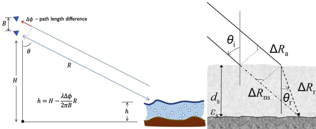
Figure 18: (a) Illustration of an interferometric viewing geometry for a vertical baseline of length, B . Using a measured path length difference measured by the interferometric phase, \Delta\phi , simple trigonometric calculations are used to estimate a precise value of the look angle, \theta , and consequently the relative height, h , of the scattering phase center compared to the reference height, H . Calculations of differential phase such as those shown above are modulo 2\pi , and hence some care should be taken to correctly estimate the absolute phase difference. (b) When the phase centre is below the snow surface, refraction in snow must also be considered. At low microwave frequencies (e.g. L-band) in dry snow, the phase centre is often the snow-ground interface, and due to the slower electromagnetic velocity in snow, phase changes are related to changes in snow depth and density.
