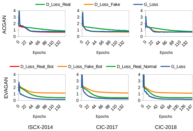
Figure 5. CC GANs Losses: The training losses for ACGAN and EVAGAN on three different CC datasets
