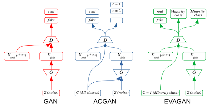
Figure 2. Comparison of EVAGAN model with vanilla GAN and ACGAN
