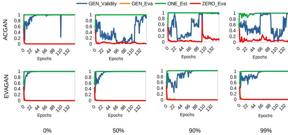
Figure 6. CV GANs estimations: The estimations on the test set for ACGAN and EVAGN for MNIST dataset in different undersampling scenarios. The range of the estimation value on the y-axis is from 0 to 1
