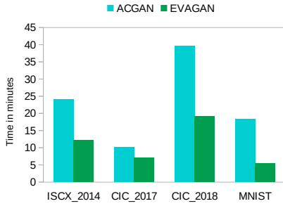
Figure 10. Time complexity
