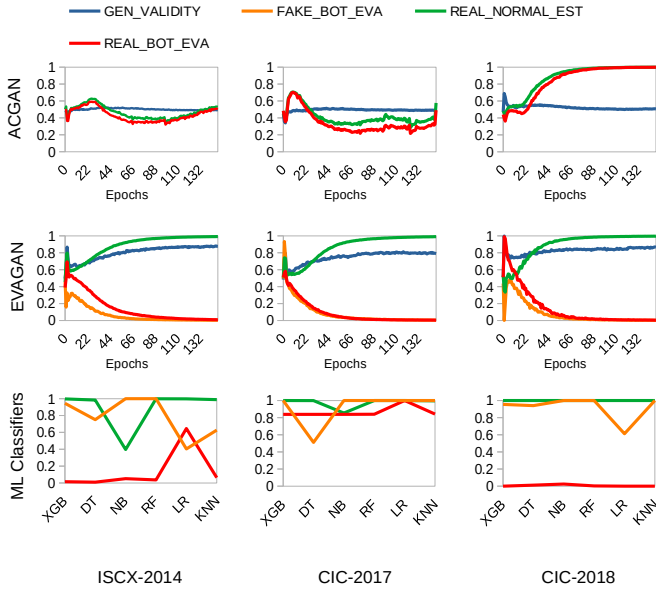
Figure 4. CC Estimations: The estimations on test data and data generated by the relative GANs along with the results of six different ML-classifiers
