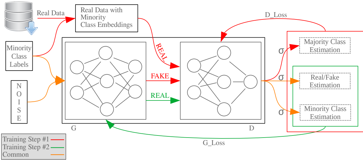
Figure 3. EVAGAN Architecture
