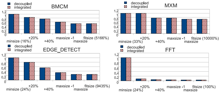
Fig. 6. Experimental results for decoupled and integrated approaches
