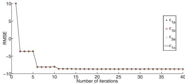
Fig. 2. NRMSE vs. iteration curves for FV denoising the image shown in Fig. 1. \epsilon_{1o} and \epsilon_{3o} correspond to the \ell_1 and \ell_2 energy of the original image. Bounds are selected \epsilon_{1a} = 0.8\epsilon_{1o} , \epsilon_{1b} = 0.6\epsilon_{1o} , and \epsilon_{3a} = 0.8\epsilon_{3o}
