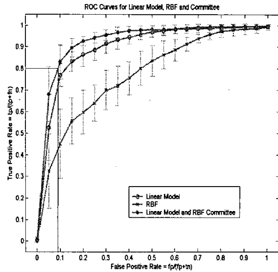
Fig. 3. Performance of Different Learning Algorithms.
