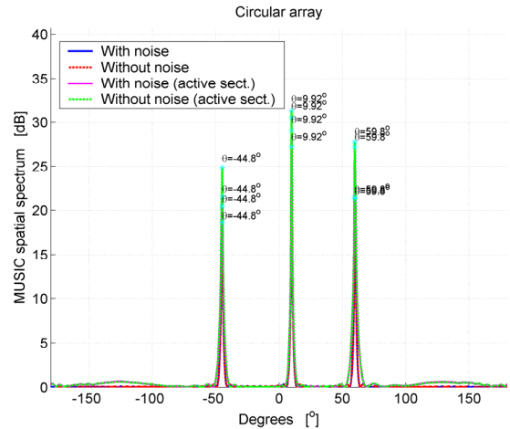
Figure 3. The MUSIC spectrum for a circular array of dipoles above a PEC cylinder.
