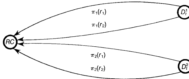
Fig. 3. Graph created by Algorithm 1.
