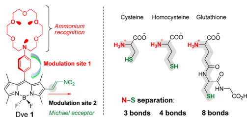
Figure 1. Structure and the signal modulation sites of the target probe. The distance between the terminal amine and the thiol suggests a much better match for GSH and the probe than the other two biological thiols.
