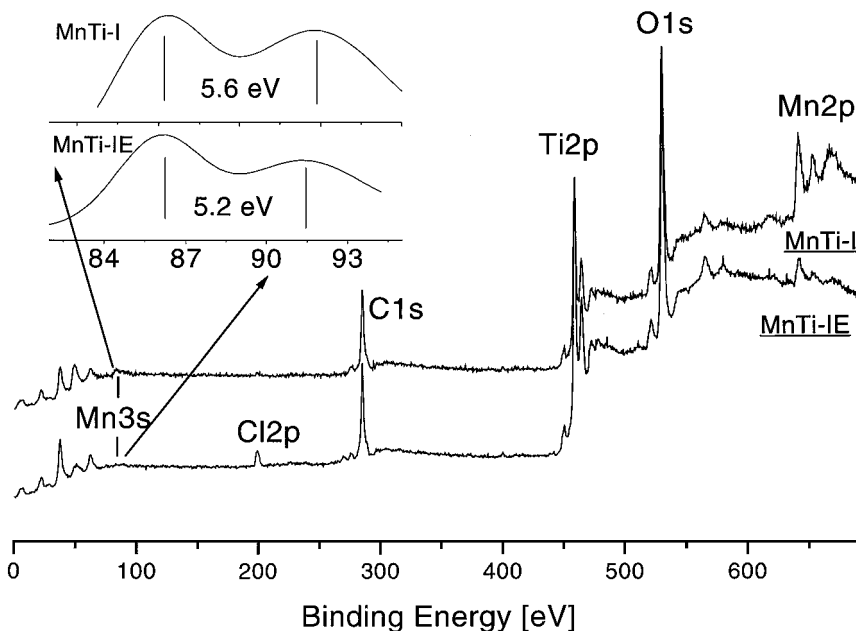
FIG. 1. X-ray photoelectron spectra of the catalysts studied.
