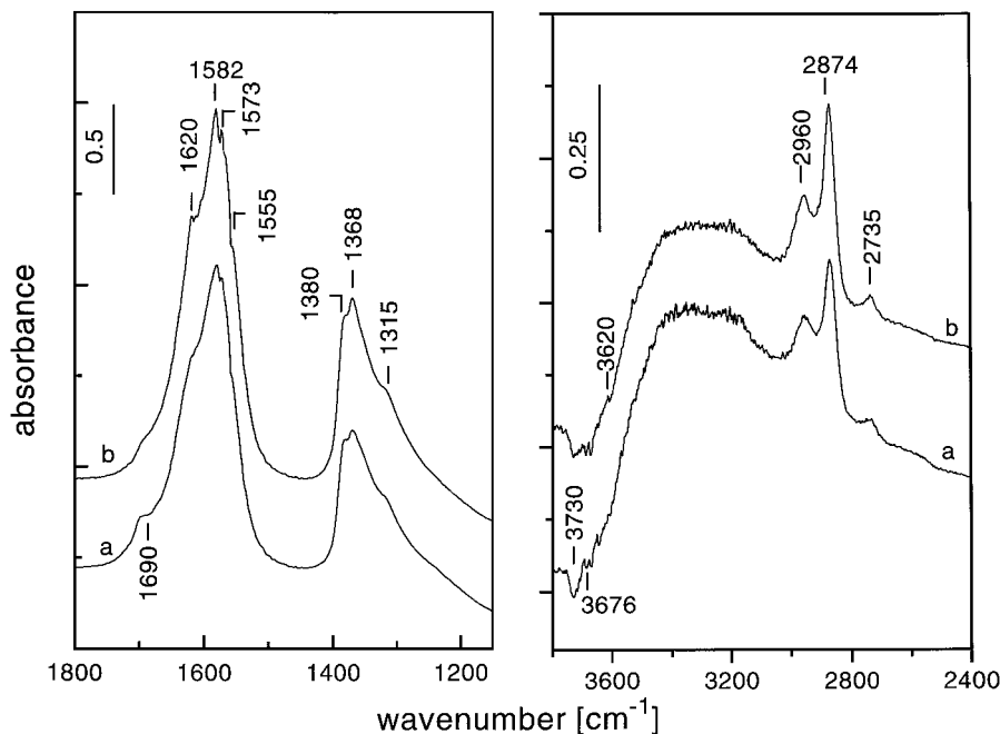
FIG. 9. FTIR spectra of adsorbed formic acid (0.5 Torr) on MnTi-IE catalyst (a) and after 10 min of evacuation at room temperature (b).
