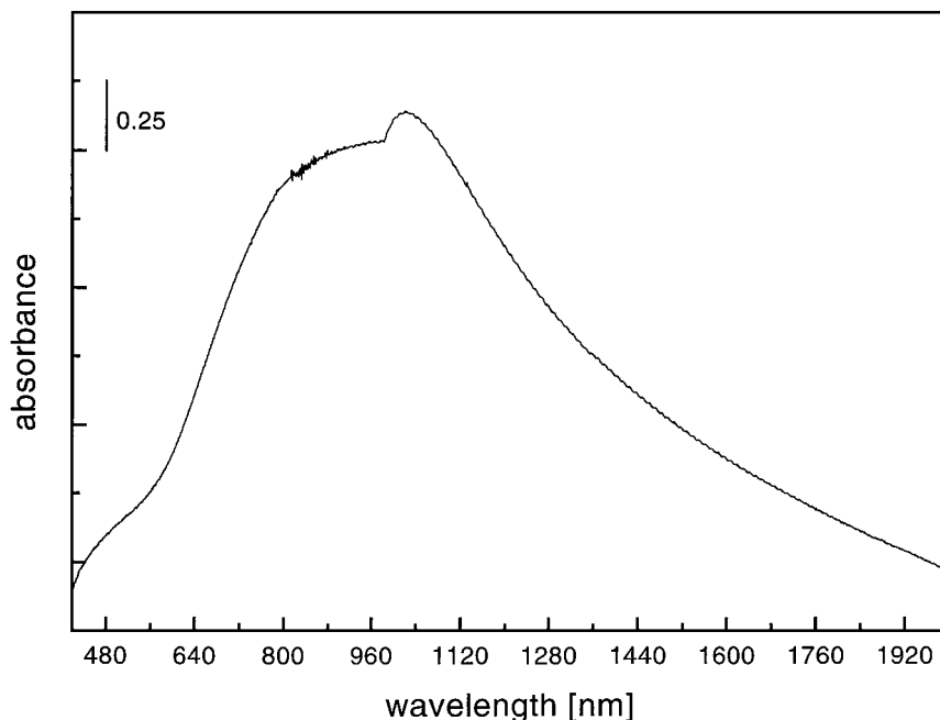
FIG. 2. Absorption spectrum in the visible range of catalyst MnTi-IE taken under ambient conditions.
