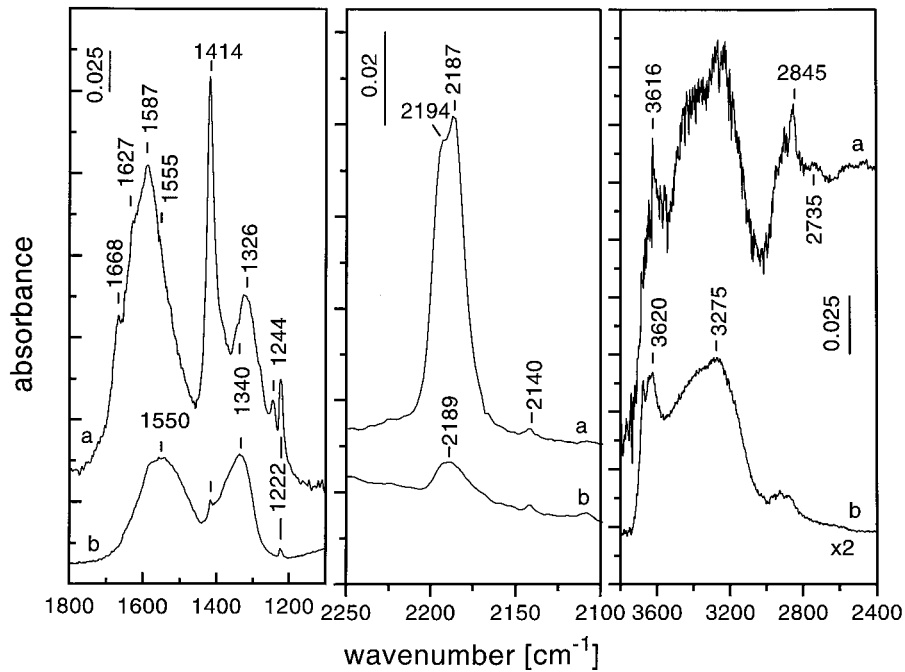
FIG. 6. FTIR spectra of adsorbed CO (30 Torr) at room temperature on MnTi-IE catalyst (a) and after reduction with hydrogen at 673 K (b).
