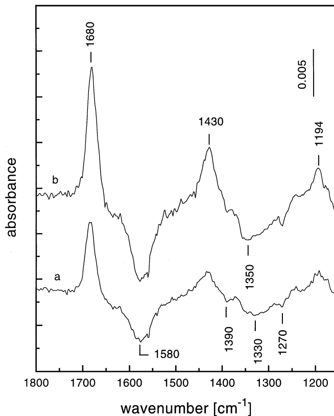
FIG. 8. FTIR spectra of partially deuterioxylated MnTi-I catalyst in the carbonate-carboxylate region obtained by subtraction of the spectrum of adsorbed CO (30 Torr) followed by evacuation for 2 min at room temperature ( p = 3.5 \times 10^{-1} Torr) from the spectrum after 4 min of evacuation ( p = 5.5 \times 10^{-3} Torr) (a) and from the spectrum after 10 min of evacuation ( p = 3.3 \times 10^{-3} Torr) (b).
