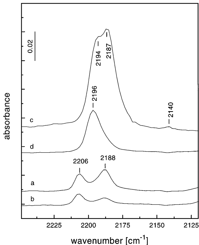
FIG. 4. FTIR spectra in the carbonyl region of adsorbed CO at room temperature on \text{TiO}_2 (anatase) at 30 Torr (a) and 1 Torr (b), and on MnTi-IE catalyst at 30 Torr (c) and 1 Torr (d).
