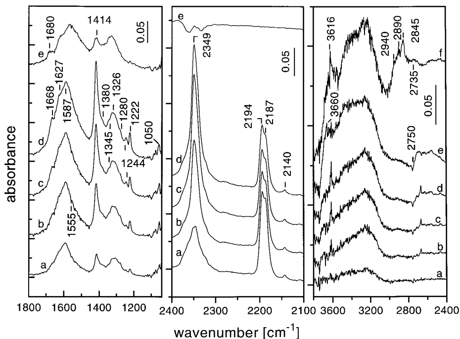
FIG. 5. FTIR spectra of adsorbed CO (30 Torr) at room temperature on partially deuteroylated MnTi-IE catalyst for various times: immediately after admission of CO to the IR cell (a); after 10 min (b); after 42 min (c); after 67 min (d); and after evacuation at room temperature for 10 min (e). The spectrum of hydroxylated MnTi-IE catalyst in the OH stretching region after 67 min in CO (30 Torr) is also shown (f).
