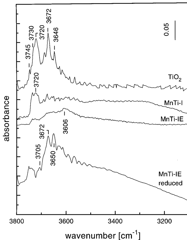
FIG. 3. FTIR spectra of the catalysts studied in the OH stretching region.
