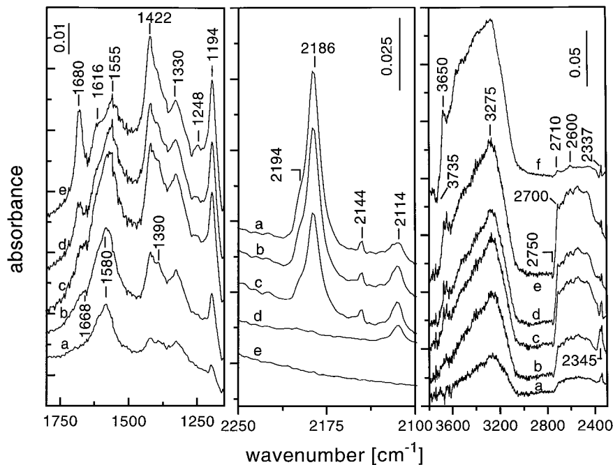
FIG. 7. FTIR spectra of adsorbed CO (30 Torr) at room temperature on partially deuterioxytated MnTi-I catalyst for various times: after 10 min (a); after 50 min (b); after 100 min (c); and after evacuation at room temperature for 2 min (residual pressure, p = 3.5 \times 10^{-1} Torr) (d) and for 10 min ( p = 3.3 \times 10^{-3} Torr) (e). The spectrum of hydroxylated MnTi-I catalyst in the OH stretching region after 67 min in CO (30 Torr) is also shown (f).
