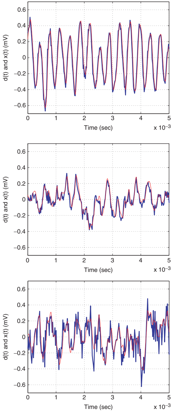
Figure 11. Timetraces of signal from cavity floor transducer (thin line) and of NN emulator response (thick line) of Mach 0.30 flow: (a) without forcing (top); (b) with optimal sinusoidal forcing at 3920 Hz, 4V_{rms} (middle); (c) white noise forcing at 6V_{rms} (bottom).
