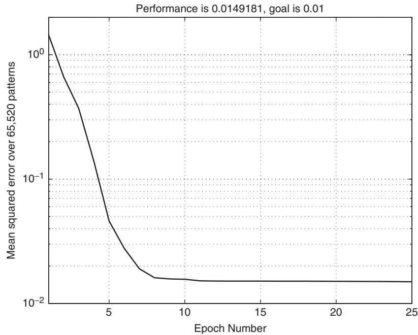
Figure 9. Time evolution of the mean squared error.
