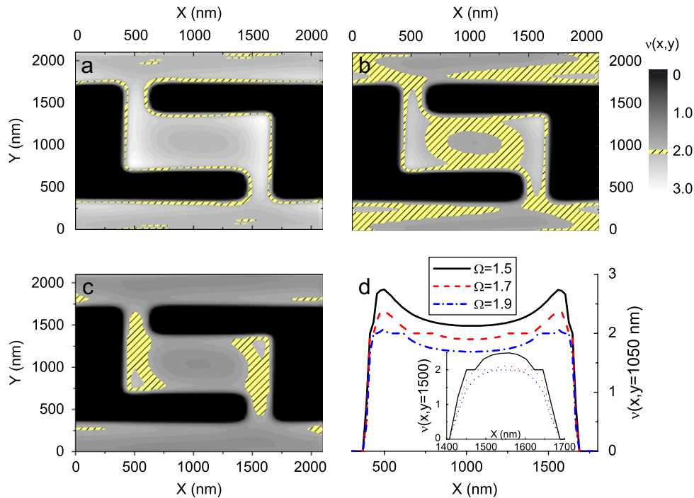
Fig. 2. (a–c) The gray scale plot of v(x,y) for three B values calculated at kT/h\omega_c = \frac{1}{40} . (d) Density cross-section again at the center (plot) and at the opening (inset).
