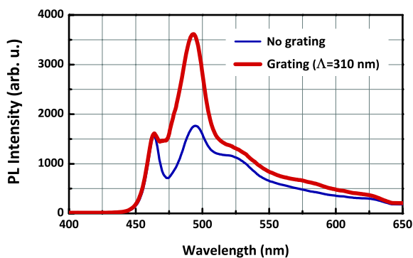
Figure 3. PL of the hybrid LED device with a grating period of 310 nm using a fiber probe for light collection.
