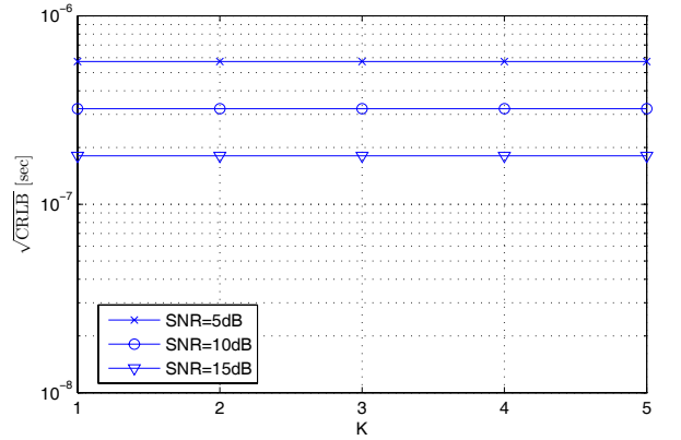
Fig. 5. \sqrt{\text{CRLB}} versus K for N = 16 and 16PSK modulation when the SNR is defined as the sum of the SNRs at different branches.
