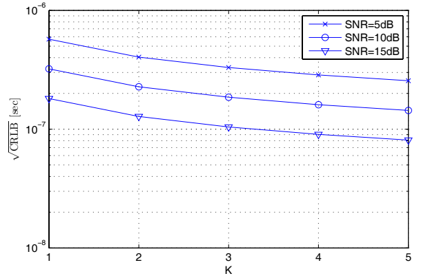
Fig. 6. \sqrt{\text{CRLB}} versus K for N = 16 and 16PSK modulation when the SNR is defined per branch.
