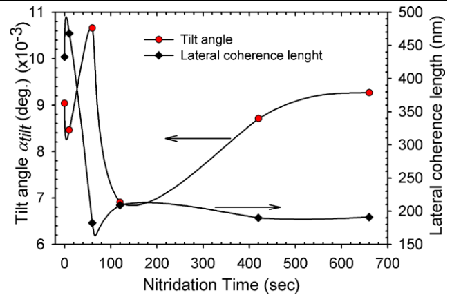
Fig. 4 Tilt and lateral coherence length obtained from the Williamson–Hall plot as a function of the nitridation time
