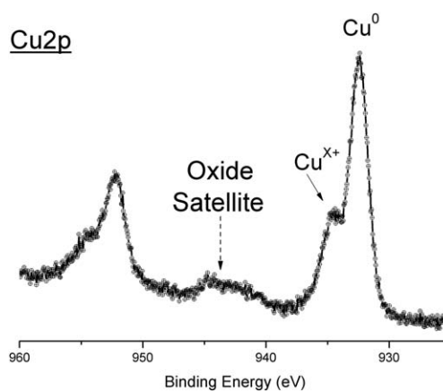
Fig. 6 Cu2p region of the XPS spectrum of AgCu nanoalloys after storing for 75 days, showing an additional CuO x satellite structure.
