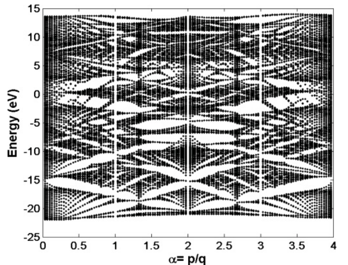
FIG. 2. The Hofstadter butterfly spectrum for graphene with all of the orbitals. Both the first- and the second-nearest-neighbor interactions are included. The tight-binding parameter are displayed in Table I.
