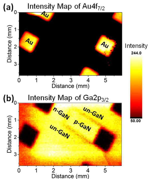
Figure 2. XPS Intensity Maps. Areal maps of the intensity of the Au4f_{7/2} and Ga2p_{3/2} peaks derived from peak areas.
