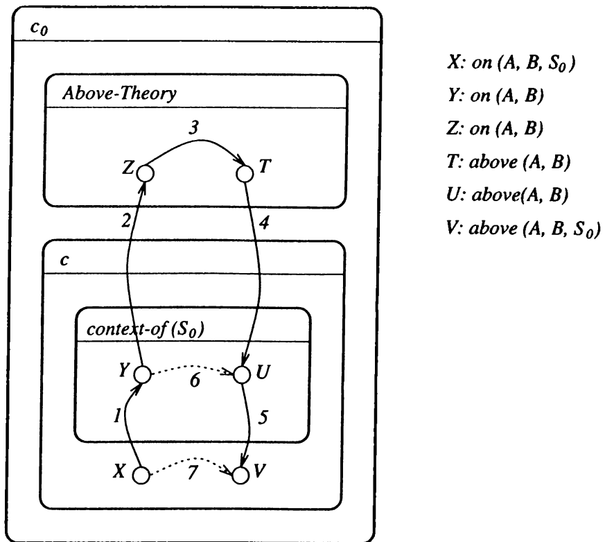
Figure 5.1. Diagram of McCarthy's proof
