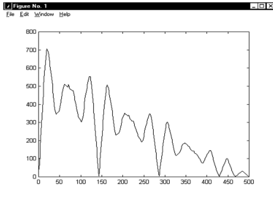
Figure 6: AMDF function for diphone “ka_b” in our database
