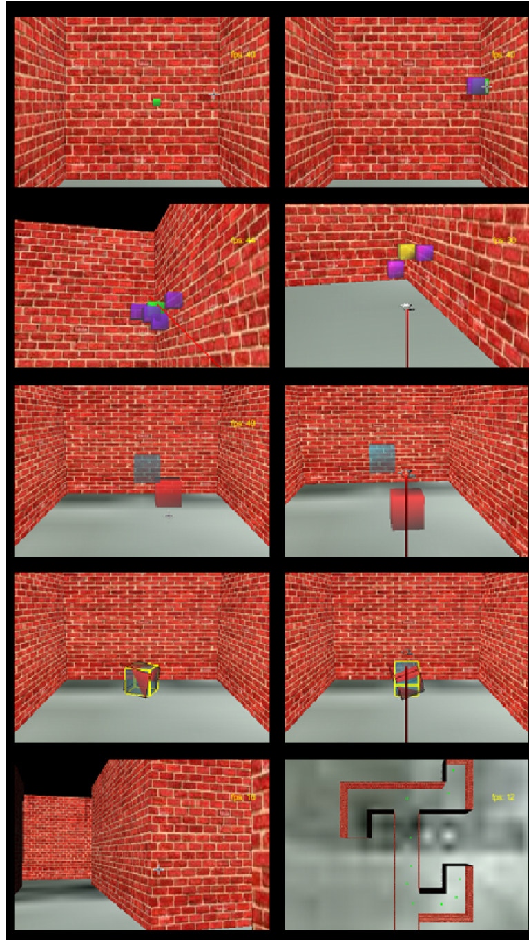
Figure 5.1: Screen captures from various test scenes, from left to right and top to bottom: Dual-Finger Midpoint Ray-Casting selecting a small object, Dual-Finger Offset Ray-Casting selecting an occluded object, Ray-Casting selecting an object from a dense environment Go-Go technique selecting an object from a dense environment, Dual-Finger Translation positioning an object on the x - z plane, Go-Go technique positioning an object, Dual-Finger Rotation and Go-Go techniques rotating an object, Dual-Finger Navigation moving and Marking Checkpoints technique planning a path in the environment.
