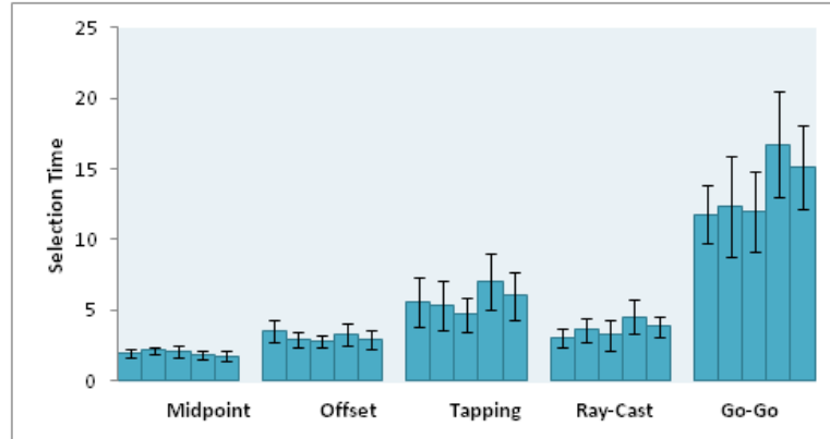
Figure 6.1: Mean selection time for each technique under different levels of target object size. The bars for each technique represent the target size for 0.25 \text{ cm}^2 , 0.2 \text{ cm}^2 , 0.08 \text{ cm}^2 , 0.04 \text{ cm}^2 and 0.01 \text{ cm}^2 respectively. Error bars represent a 95% confidence interval.
