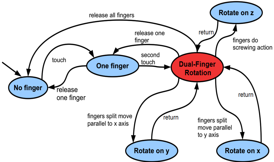
Figure 4.4: State diagram for Dual-Finger Rotation technique.
