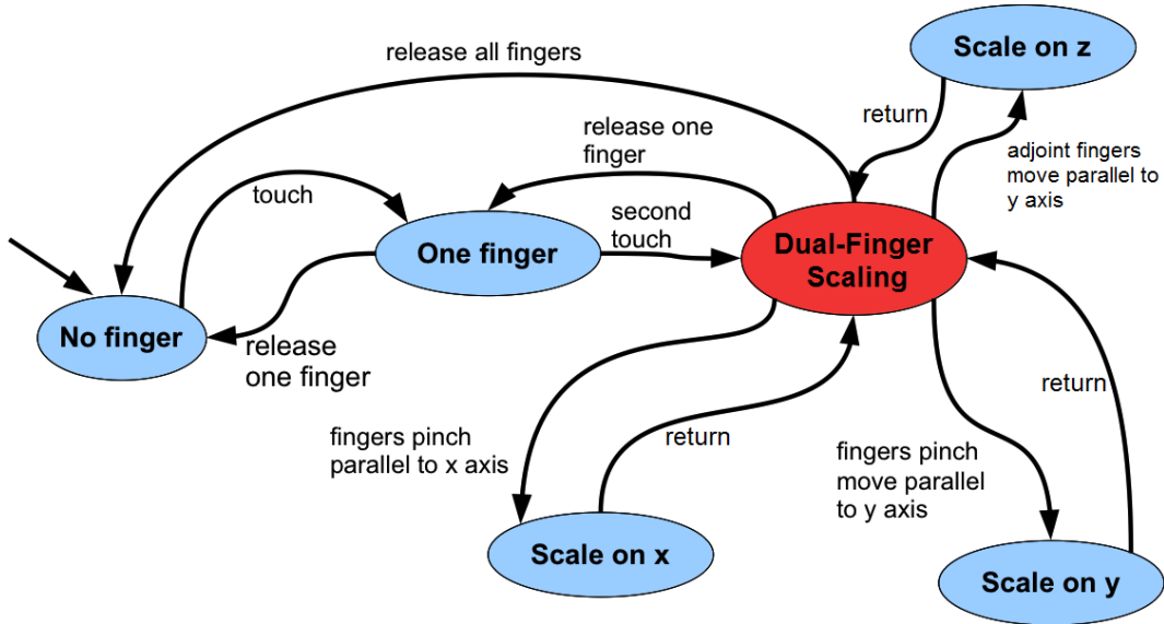
Figure 4.5: State diagram for Dual-Finger Scaling technique.
