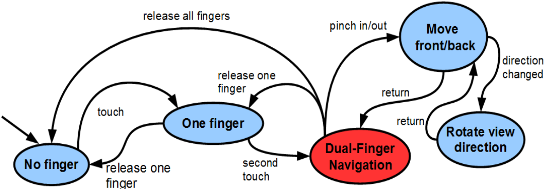
Figure 4.6: State diagram for Dual-Finger Navigation technique.
