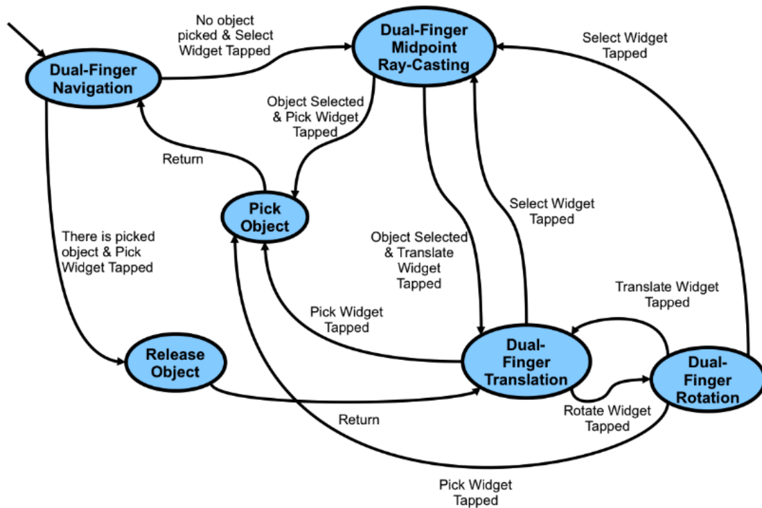
Figure 7.2: State diagram for UI Widgets Based Multi-Mode Direct Manipulation.
