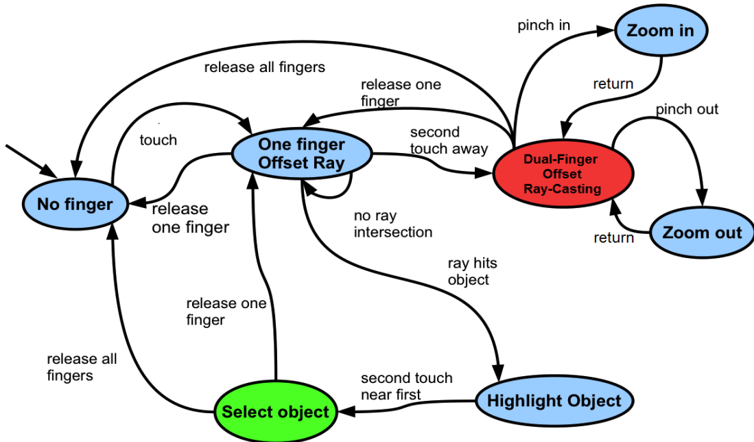
Figure 4.2: State diagram for Dual-Finger Offset Ray-Casting technique.
