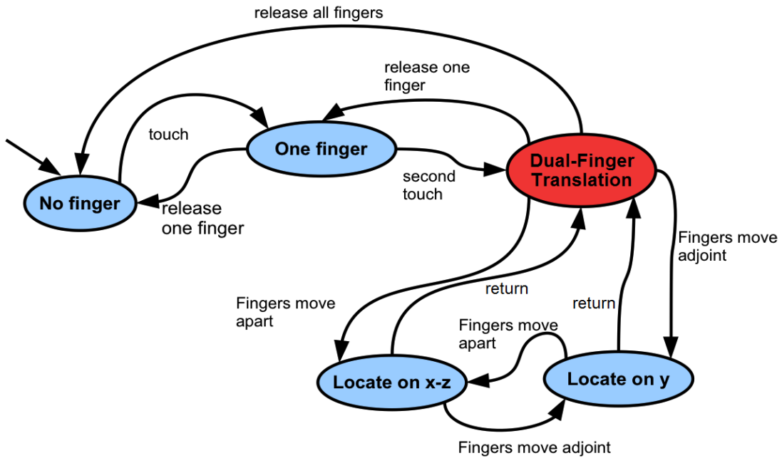
Figure 4.3: State diagram for Dual-Finger Translation technique.
