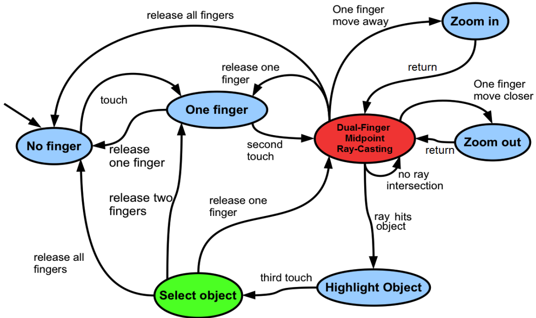
Figure 4.1: State diagram for Dual-Finger Midpoint Ray-Casting technique.
