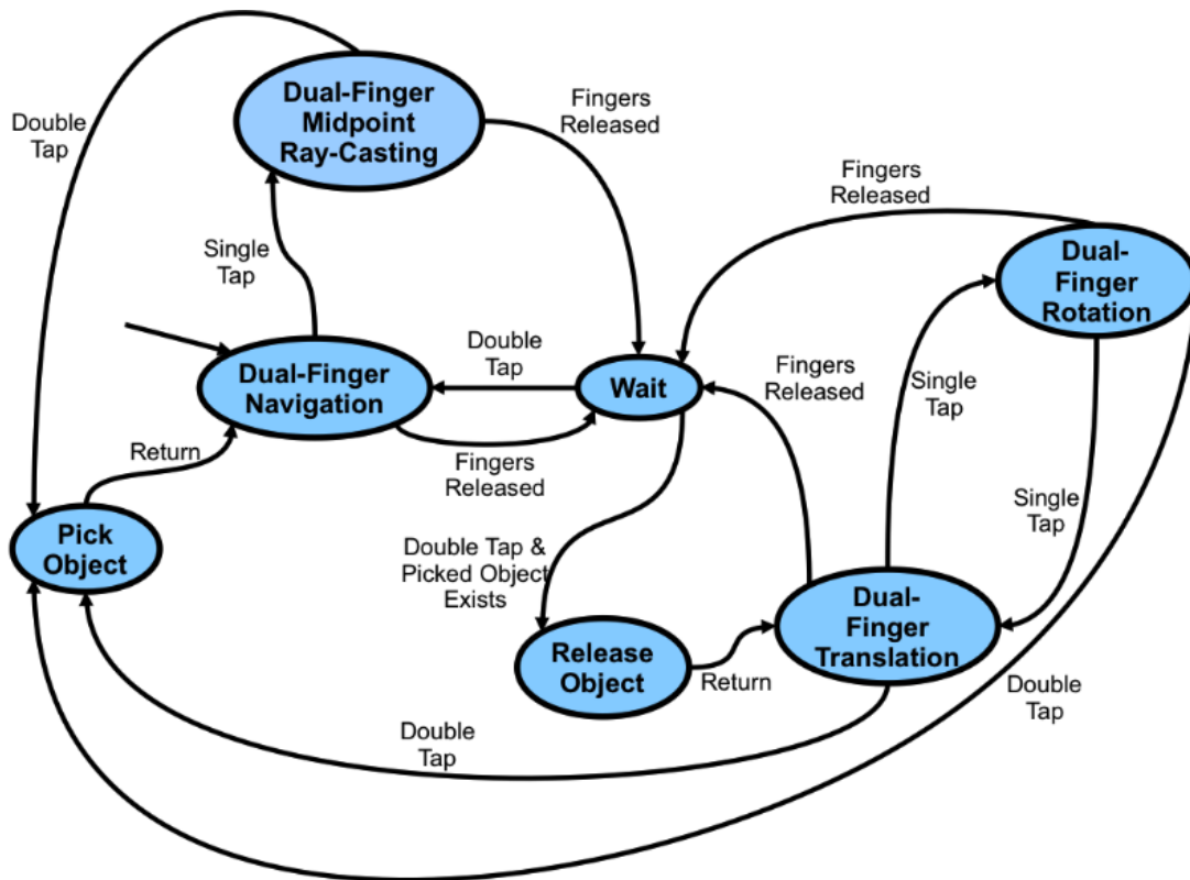
Figure 7.1: State diagram for Touchscreen Gesture Based Multi-Mode Direct Manipulation.
