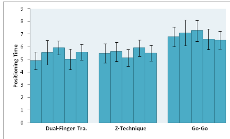
Figure 6.4: Mean object positioning time for each technique under different levels of task complexity. The bars for each technique represent task complexity, with the distance between the selected object and the target container as 1.8, 2.3, 2.9, 3.1 and 4.5 units in the 3D scene, respectively. Error bars represent a %95 confidence interval.
