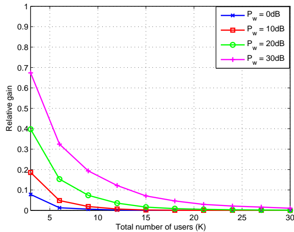
Figure 4.4: Relative gain in sum rate over noncooperative scheme under MSR scheduling.
