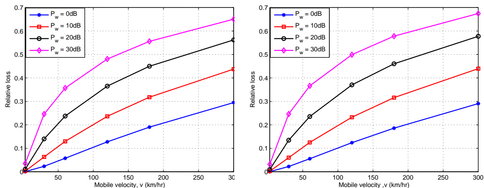
(a) Noncooperative transmission strategy. (b) Cooperative transmission strategy.
