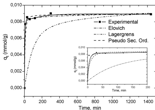
Fig. 3. Variation of the adsorbed amount of Ba 2+ with time as revealed by the experimental data in comparison to Lagergren's, Elovich, and pseudo-second-order model predictions. The inset figure shows the variation of adsorbed amount at the earlier stage of adsorption.
