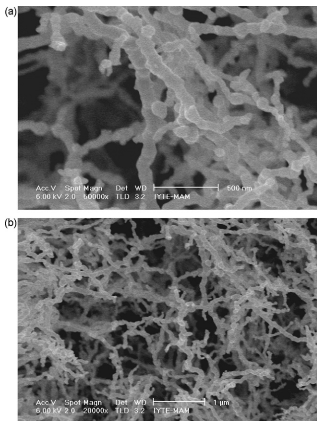
Fig. 2. SEM images of iron obtained at magnification of: (a) 50 000 \times and (b) 20 000 \times .
