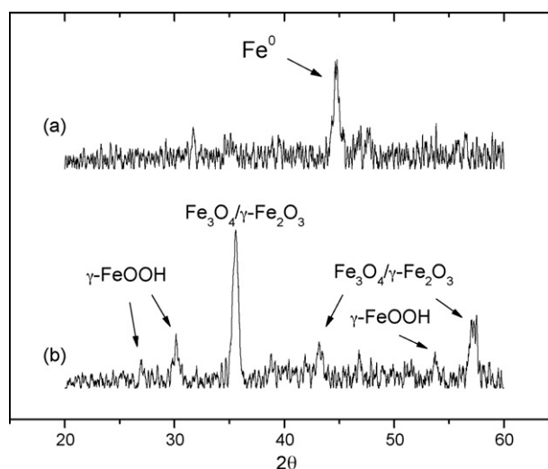
Fig. 1. XRD patterns of iron nanoparticles: (a) before adsorption and (b) after adsorption of \text{Ba}^{2+} ions.
