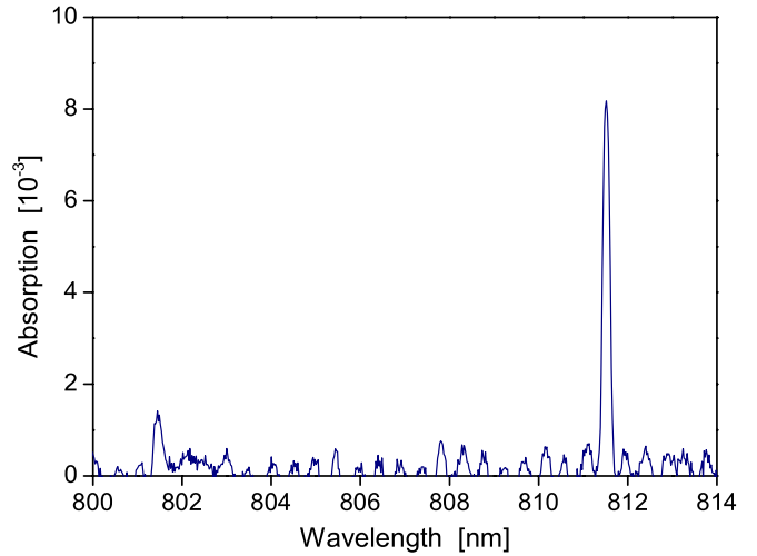
Figure 6. Absorption spectrum around the argon transitions at 801.5 and 811.5 nm.
