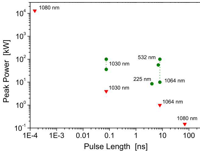
Figure 8. Parameter diagram for successful (green circles) and unsuccessful (red triangles) breakdown attempts in dependence of wavelength, pulse length and peak powers. Right: Sketch of the experimental setup for laser assisted plasma breakdown.
