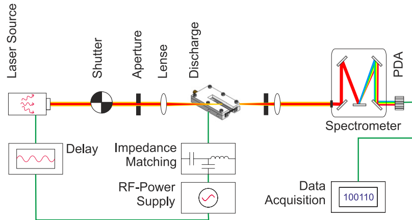
Figure 2. Experimental setup for broad-band absorption measurements with supercontinuum or LED light source.
