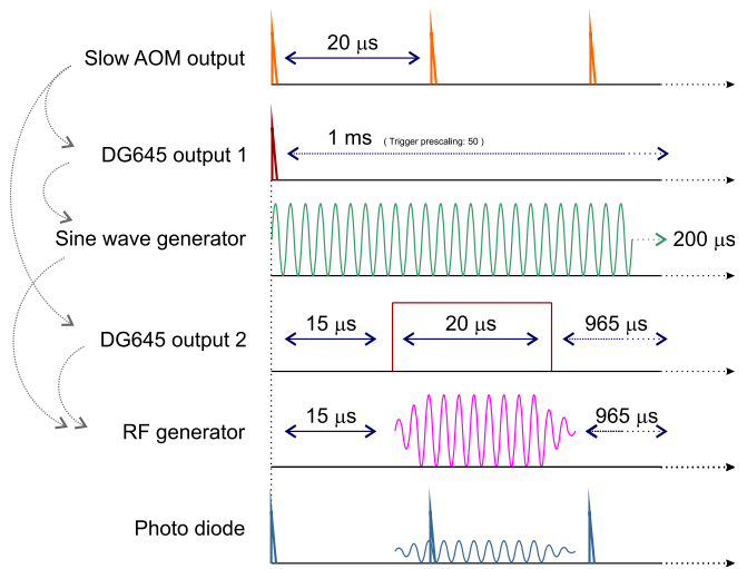
Figure 9. Trigger sequence for phase locked operation of fibre laser and RF generator. AOM = acousto-optic modulator, DG645 = delay generator.
