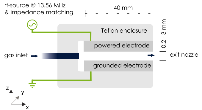
Figure 1. Scheme of the micro-plasma jet discharge.
