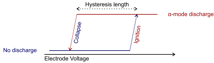
Figure 7. Discharge ignition and collapse hysteresis of the micro-plasma jet.
