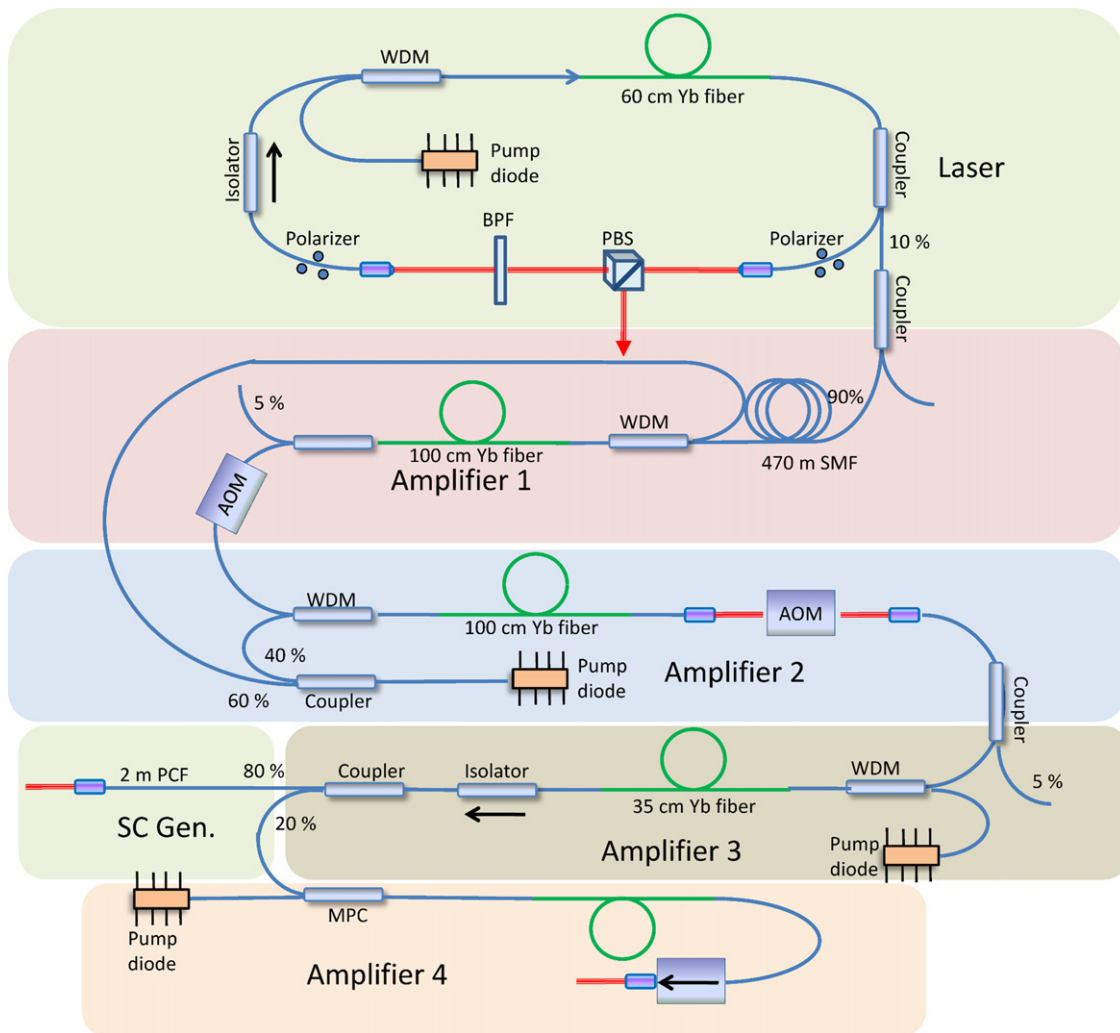
Figure 3. Fibre laser setup for supercontinuum and high-power pulse generation. WDM = wavelength-division multiplexing, PCF = photonic crystal fiber, MPC = multiport pump signal combiner.
