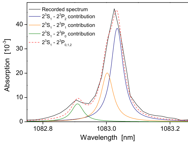
Figure 5. Absorption spectrum around the \text{He}^m 2^3\text{S}_1 \rightarrow 2^3\text{P}_J^0 ( J = 0, 1, 2 ) transitions at 1083 nm (black line). Recorded with a spectrometer featuring 75 cm focal length, a 1200 lines per mm grating and few \mu\text{m} slit opening, together with a photo diode array as detector. Also displayed are three Voigt functions, representing the respective transitions from the \text{He}^m 2^3\text{S}_1 level. The functions have been modelled with the results obtained by TDLAS measurements (line width and position) and show perfect agreement with the BBAS measurements.
