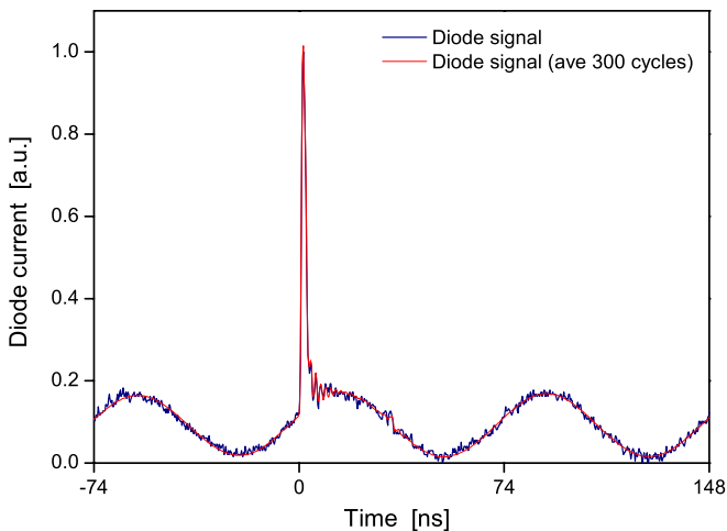
Figure 10. Current signal of a photo diode placed behind the discharge. The current shows the laser pulses as well as the RF signal that is phase locked to the laser.
