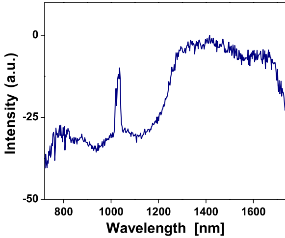
Figure 4. Spectral profile of the supercontinuum beam (logarithmic scale).
