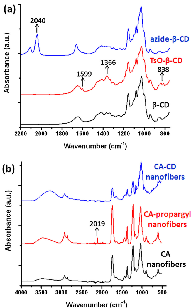
Fig. 2. (a) FTIR spectra of \beta -CD, TsO- \beta -CD and azide- \beta -CD powder, (b) ATR-FTIR spectra of CA, CA-propargyl and CA-CD nanofibers.
