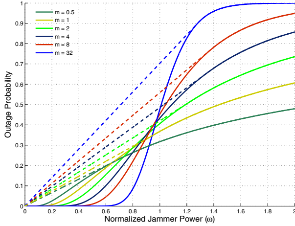
Fig. 5. Outage probability versus normalized jammer transmit power for fixed power jamming (solid lines) and optimum jammer power randomization (dashed lines) for various values of fading parameter m .
