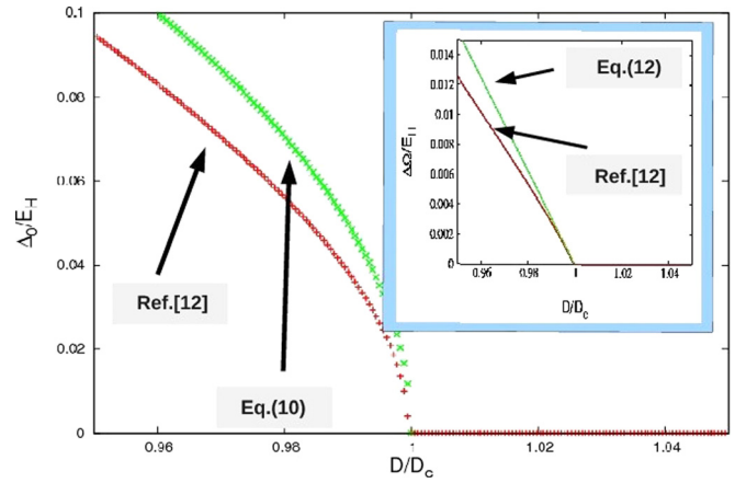
FIG. 1. Comparison of Ref. 12 with Eqs. (10) and (12) as D is varied near D_c . The main figure depicts \Delta_0/E_H and the inset is \Delta\Omega/E_H , where E_H = e^2/(4\pi\epsilon a_B) and a_B = \hbar^2 4\pi\epsilon/(e^2 m_x) . (The numerical solution includes the self energies as well as their realistically different masses.)
