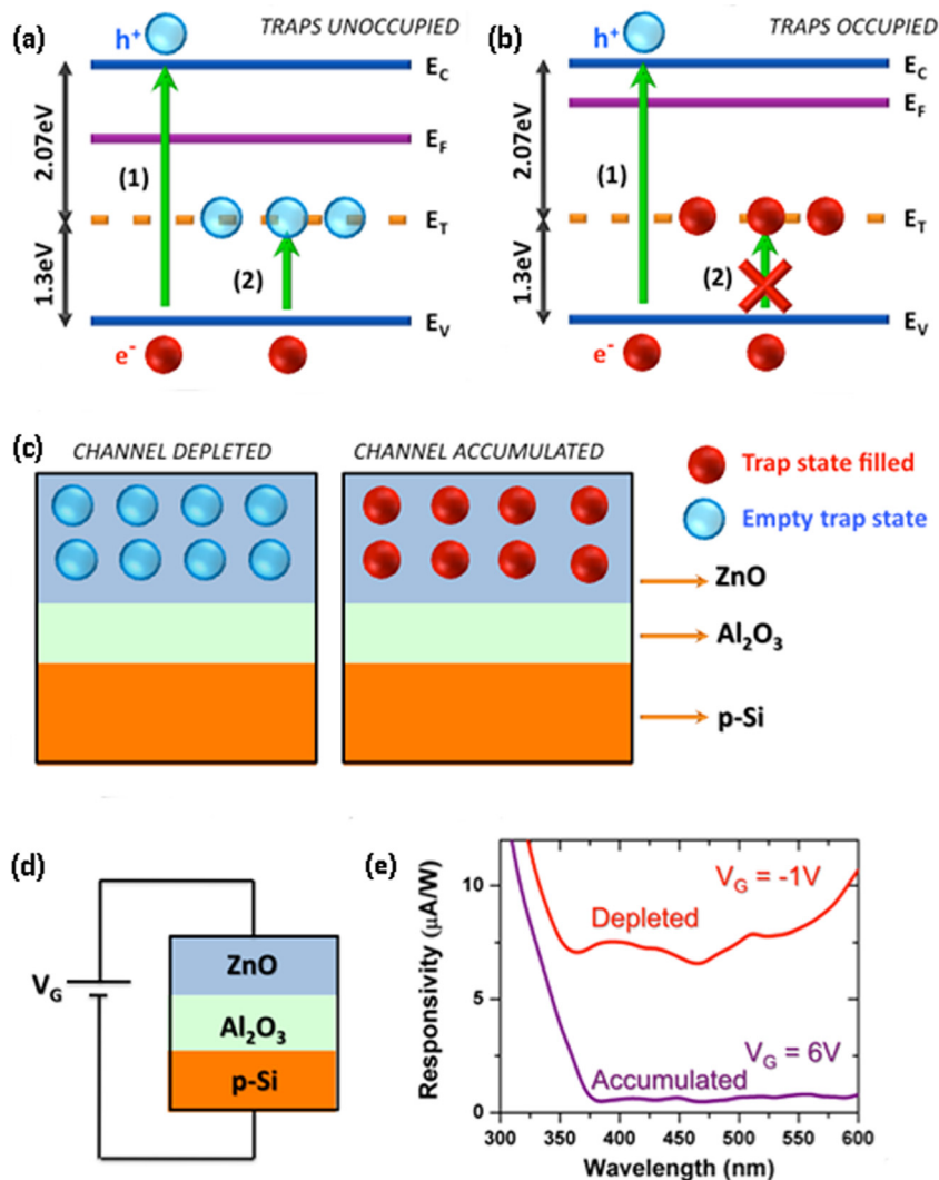
FIG. 6. (Color online) Trap related optical characteristics of ZnO deposited at 80^{\circ}\text{C} . Energy band diagram depicting trap states (a) unoccupied and (b) occupied by an electron. Band-to-band (1) and valence band-to-trap state (2) absorption mechanisms are shown by arrows. When the traps are occupied, second transition is suppressed. (c) Illustration of the MOS gate sketch of TFT devices comprised of p-Si/ \text{Al}_2\text{O}_3 /ZnO. ALD-grown ZnO is the channel layer. (d) Applied gate bias voltage and measured spectral photoresponsivity at accumulated state ( V_G = 6\text{ V} ) and depleted state ( V_G = -1\text{ V} ).
