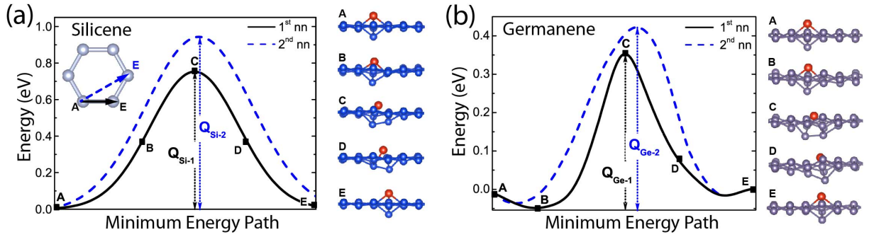
Figure 7: (a) Migration of Si-DB on silicene and (b) Ge-DB on germanene. Energetics and the migration energy barrier ( Q ) of a single, isolated DB between the first and second nearest neighbors are shown by the inset in the left panel. The barriers are calculated using the nudged elastic band (NEB) method. Snapshots of the atomic configurations taken at stages A, B, C, D and E during the migration of DB to the first nearest neighbor site are also presented to illustrate the mechanism of diffusion.
