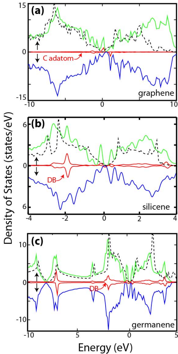
Figure 3: Total density of states for (a) C on graphene (b) Si on silicene and (c) Ge on germanene. The partial DOS of the adatoms are indicated by red lines and multiplied by a factor of 2 for better visualization. Spin up and spin down states are shown with green and blue lines, respectively. DOS of pure graphene, silicene and germanene are also indicated by the dashed curves in the plots.
