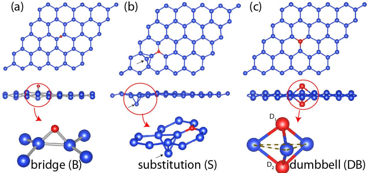
Figure 1: Side and top views of various types of equilibrium atomic structures, which occur when a Group IV element (C, Si, Ge and Sn) is adsorbed on the single layer honeycomb structure constructed from Group IV elements (graphene, silicene and germanene). (a) A Group IV adatom adsorbed at the bridge site, i.e. B-site. (b) Substitution of silicene or germanene host atoms by the carbon adatom, i.e. S-site. The small arrows indicate the host Si atom that is pushed down after the substitution of C adatom. (c) Dumbbell structure (DB) constructed by Si, Ge and Sn adatoms adsorbed on silicene and germanene. D_1 and D_2 are dumbbell atoms; D_1 is the adatom, D_2 is the host atom pushed down by D_1 . Adatom and single-layer substrate atoms are described by red and blue balls, respectively.
