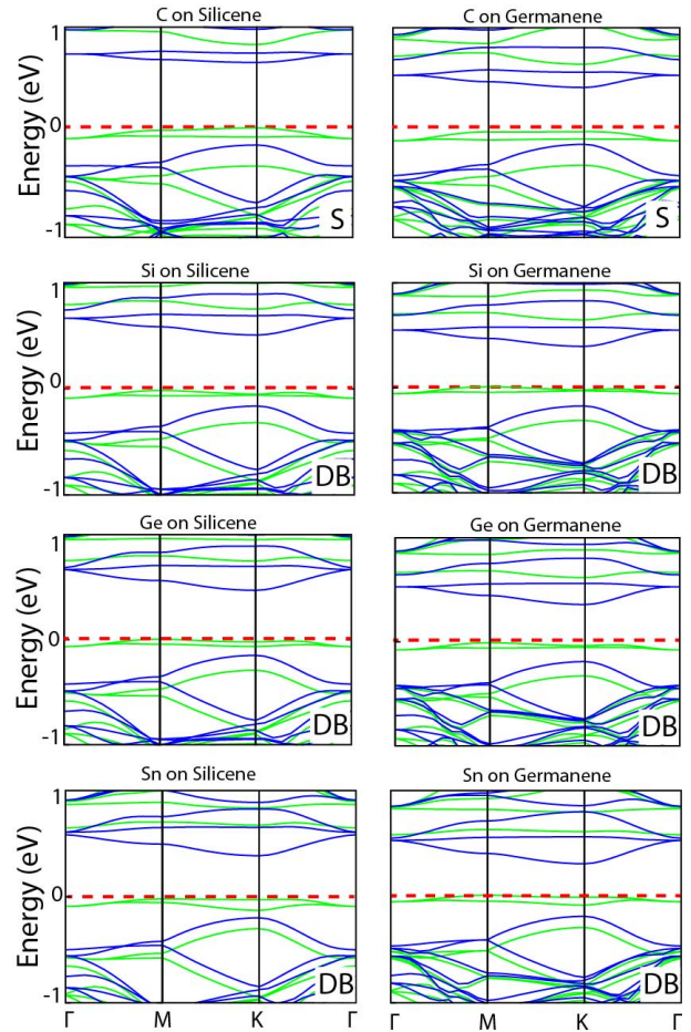
Figure 5: Electronic band structures are calculated by using HSE for single layer silicene and germanene with adatoms C, Si, Ge and Sn, which form a 5 \times 5 supercell or pattern. In the spin polarized systems, spin up and spin down bands are shown with green and blue lines. The zero of energy shown by red dashed line is set to the energy of highest occupied state. Binding structures (as B, S, DB) are indicated in each panel.
