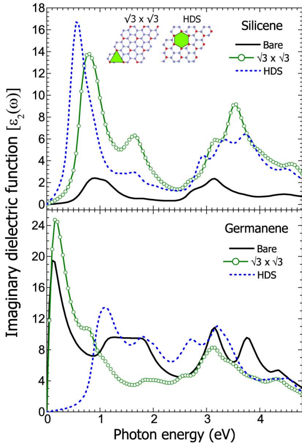
Figure 6: The optical absorption spectra of bare (black curve), (\sqrt{3} \times \sqrt{3}) (green curve with dots) and HDS (dashed blue curve) structures of silicene (top) and germanene (bottom), respectively. Structures are shown in the inset plots.
