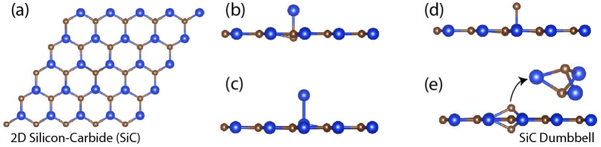
Figure 2: Equilibrium binding structures of C and Si adatoms on graphene like structure of SiC. (a) Top view of compound SiC displaying a planar honeycomb structure. (b) Si adatom on C host atom; (c) Si adatom on Si host atom; (d) C adatom on Si host atom are adsorbed at the head-on positions rather than forming a dumbbell structure. (e) C adatom on host C atom of SiC forming a DB structure. Si and C atoms are indicated by large blue and small brown balls, respectively.
