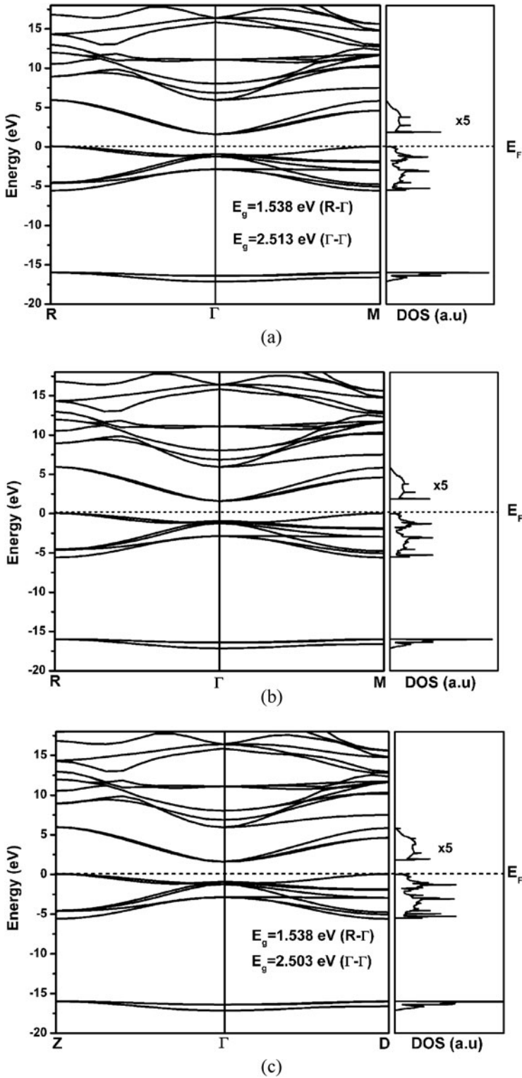
Figure 1. Electronic band structure and DOS of KNbO 3 , cubic (a), tetragonal (b), rhombohedral (c).
