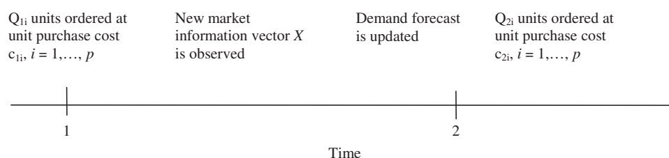
Fig. 1. The ordering decisions in the model.
