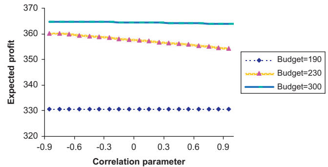
Fig. 4. Effect of correlation parameter \rho on expected profit at different budget levels in the two-product problem.
