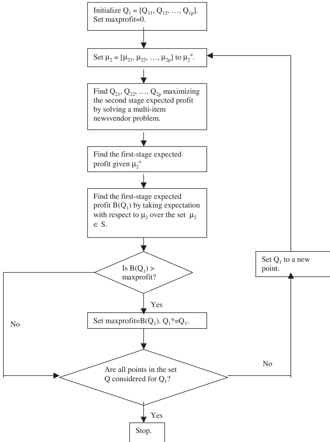
Fig. 2. Solution procedure for the budget-constrained multi-product problem.
