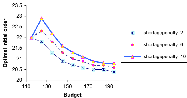
Fig. 3. Effect of shortage penalty \pi on optimal initial order at different budget levels in the single-product problem.
