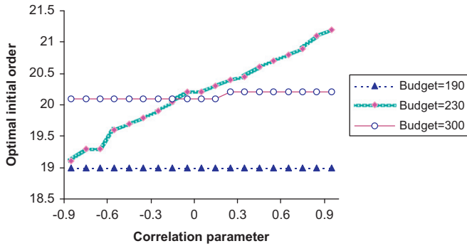
Fig. 5. Effect of correlation parameter \rho on optimal initial order at different budget levels in the two-product problem.
