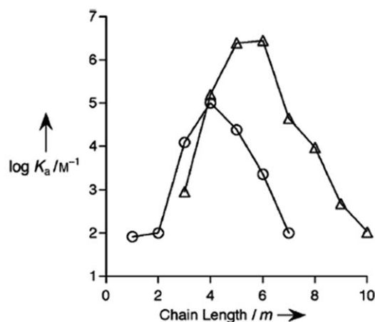
Figure 2. Relationship between the binding constant ( \log K_a ) versus chain length m for \text{H}(\text{CH}_2)_m\text{NH}_3^+ (O) and ^+\text{H}_3\text{N}(\text{CH}_2)_m\text{NH}_3^+ ( \Delta ). [17]
