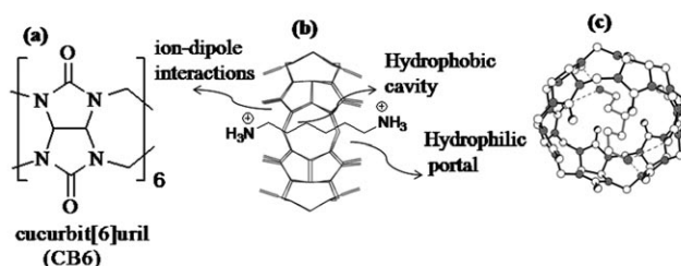
Figure 1. (a) Chemical structure of CB6 (left), (b) representation of the different binding regions of CB[6] and the geometry of the complex between CB6 and the hexanediammonium ion, (c) X-ray crystal structure of the inclusion complex of CB6 with 1,6-diaminohexane dihydrochloride salt (right). [13]
