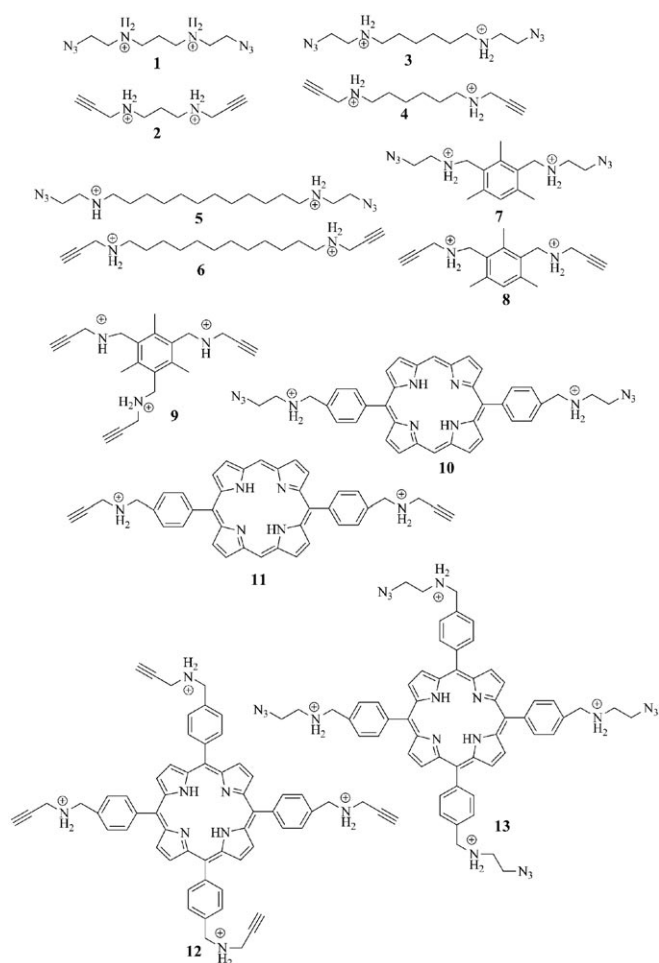
Figure 4. Structures of monomers used in the synthesis of various supramolecular assemblies. Chloride counterions have been omitted for clarity.
