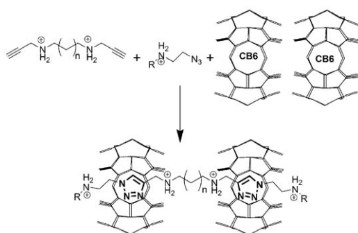
Figure 7. Synthesis of [3]pseudorotaxanes P1 ( R=H , n=1 ) and P2 ( R=H , n=10 ) and [3]rotaxanes R1 ( R=tBu , n=1 ) and R2 ( R=tBu , n=10 ) from monomers 2 ( n=1 ) and 6 ( n=10 ). Chloride counterions have been omitted for clarity.
