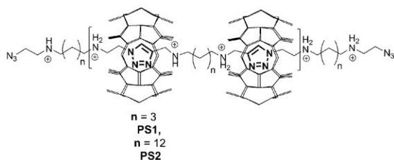
Figure 6. The structures of polyrotaxanes PS1 and PS2 . PS1 from monomers 1 and 2 , and PS2 from monomers 5 and 6 were synthesized using CB6 as a macrocycle and catalyst. Chloride counterions have been omitted for clarity.
