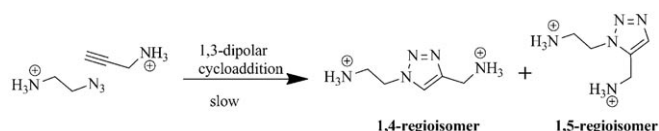
Scheme 1. The azide-alkyne Huisgen 1,3-dipolar cycloaddition reaction.
