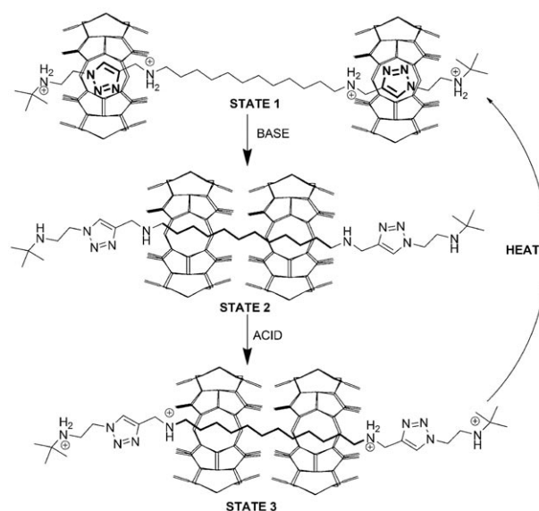
Figure 8. The pH and heat-induced shuttling processes of R2 .
