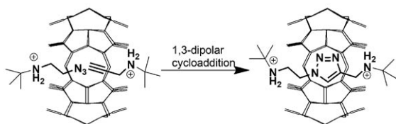
Figure 3. Synthesis of [2] rotaxane by CB6-catalyzed 1,3-dipolar cycloaddition.
