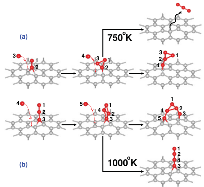
FIG. 9. (Color online) Schematic description of irregular growth of CACs, when the distance between a CAC and C* becomes accidentally close to \sim 1.50 Å. (a) C* and C 2 form a triangular cluster, which is attached to the top site from its corner. Thereafter CACs can grow regularly if additional C* approaches the triangular cluster no closer than 2.1 Å. At 750 K, the triangular cluster is removed from the graphene and, subsequently, it transforms to free-standing linear CAC in vacuum. (b) Irregular growth of a quadrangle formed from CAC(3) and C* and adsorbed at the bridge site under similar conditions as (a). Irregularity may continue in the next growth step, but at 1000 K a quadrangle cluster can transform to the linear CAC(4).
