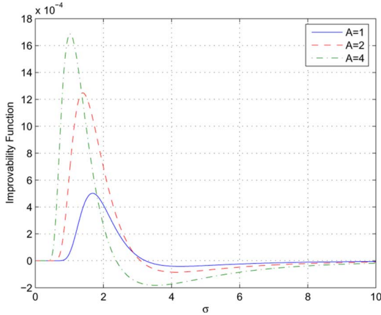
Fig. 1. Improvability function obtained from Proposition 3 for various values of A , where \rho_1 = 0.1 , \rho_2 = 0.2 , \mu_1 = 2 , and \mu_2 = 3 .
