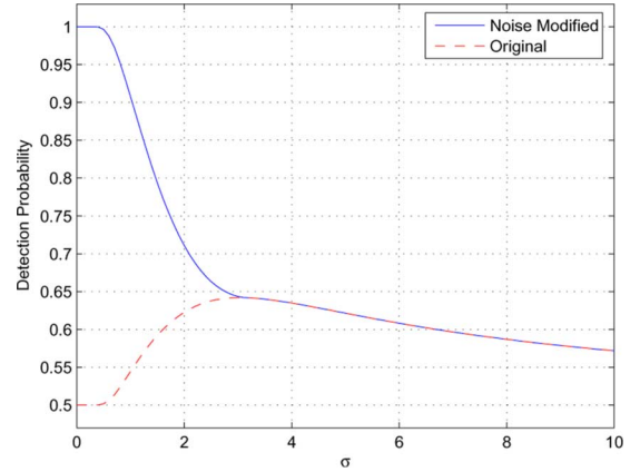
Fig. 2. Detection probabilities of the original and noise modified detectors versus \sigma for A = 2 , \rho_1 = 0.1 , \rho_2 = 0.2 , \mu_1 = 2 , and \mu_2 = 3 .
