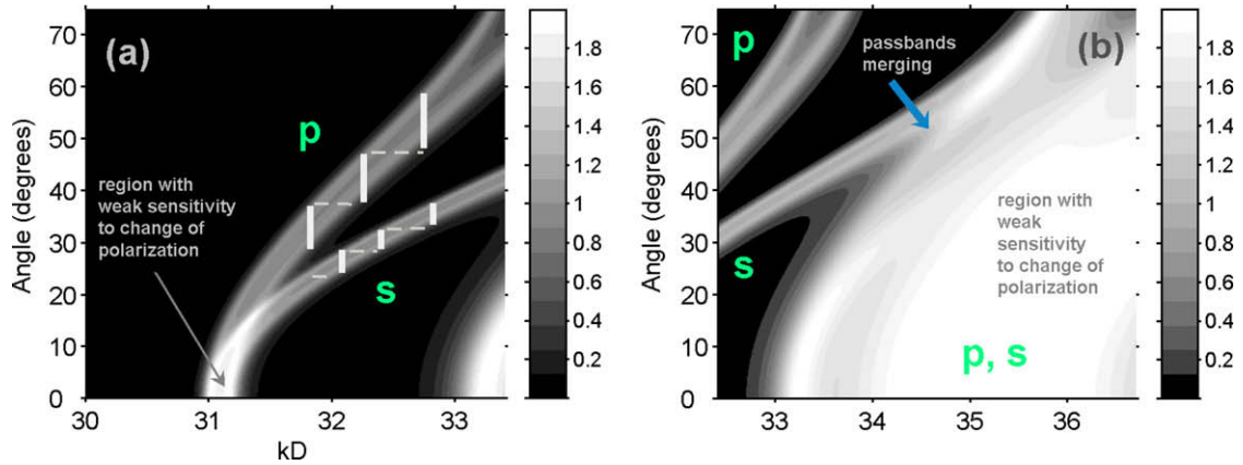
Fig. 4. Transmission for the slab with M = 21 , h = 2 , m_1 = 6 and m_2 = 16 in units of t = \mathcal{T}_s + \mathcal{T}_p vs kD and \theta at (a) kD varied from 30 to 33.4, and (b) kD varied from 32.4 to 36.7; non-overlapping pass bands are shown in plot (a) by dashed lines.
