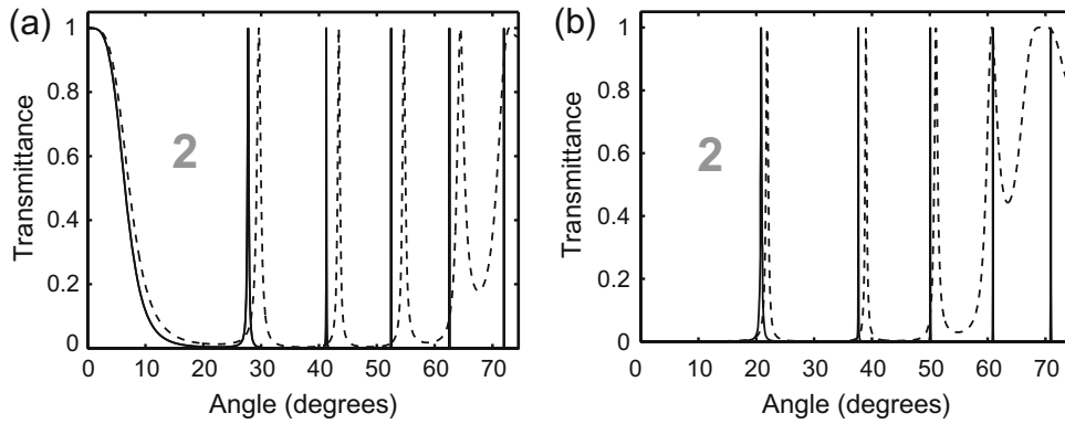
Fig. 6. Polarization-sensitive transmission within multiple narrow pass bands at M = 16 , h = 6 , m_1 = 6 , m_2 = 7, \dots, m_6 = 11 ; (a) kD = 53.88 , (b) kD = 52 ; Solid lines - s polarization, dashed lines - p polarization.
