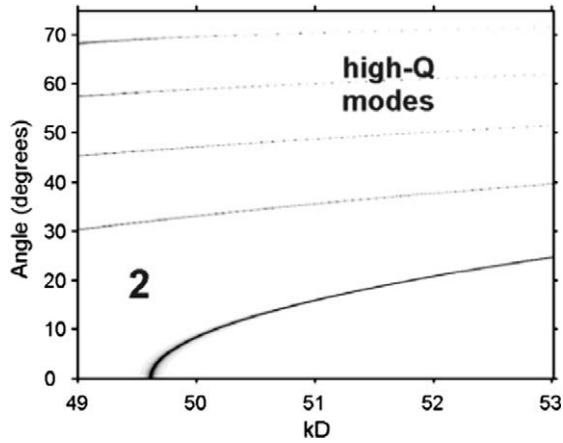
Fig. 7. Transmission vs kD and \theta for the slab with M = 16, h = 6, m_1 = 6, m_2 = 7, \dots, m_6 = 11, s polarization; the most dark tone in the middle of every line (trace) corresponds to \mathcal{T}_s = 1 .
