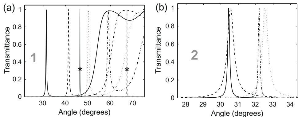
Fig. 8. Transmittance at M = 16, h = 6, m_1 = 6, m_2 = 7, \dots, m_6 = 11 ; Case (a) – solid lines: kD = 23.5 , dashed lines: kD = 24 , dotted line: kD = 24.51 , and dash-dotted line: kD = 25.05 ; lines without asterisk – p polarization, lines with asterisk – s polarization; Case (b) – solid line: kD = 49, s polarization; dashed line: kD = 49, p polarization; dash-dotted line: kD = 49.61, s polarization; dotted line: kD = 49.61, p polarization.
