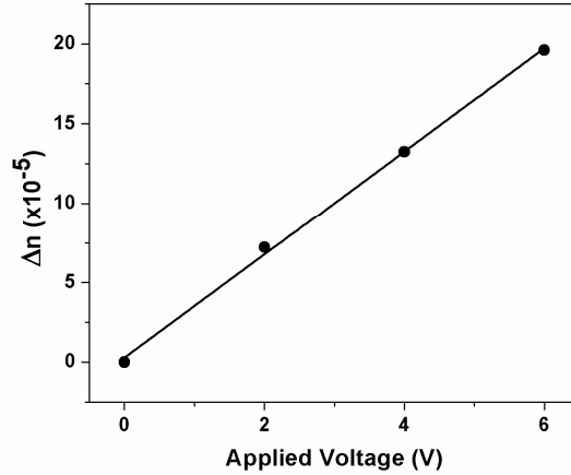
Fig. 3. Variation in refractive index as a function of applied voltage at 1515 nm. The dots show the experimental data and the line indicates the linear fit.
