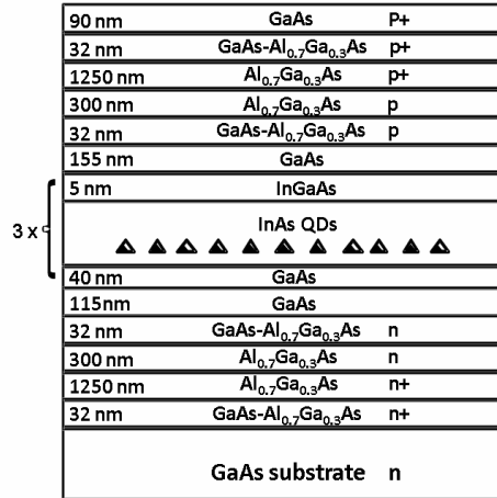
Fig. 1. Detailed structure of the samples used in the measurements. \text{Al}_{0.7}\text{Ga}_{0.3}\text{As} layers at the GaAs interfaces are graded.
