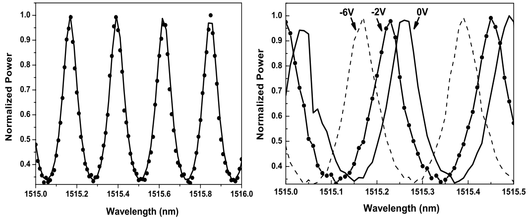
Fig. 2. (a) Fabry-Perot resonances at 1515 nm for 6 Volt reverse bias. The dots show the experimental data and the line indicates the optimum curve fit. (b) Voltage dependent shift of Fabry-Perot resonances. Significant tuning is observed with relatively low voltages.
