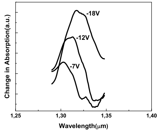
Fig. 4. Change in absorption due to applied reverse bias. Red shift of the spectra should be noted with increasing applied voltage.
