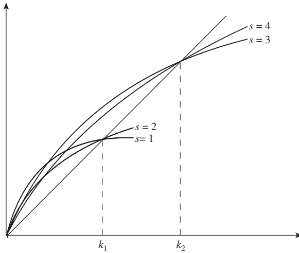
Fig. 2. \Omega_1 = \{1, 2\} , \Omega_2 = \{3, 4\} .
