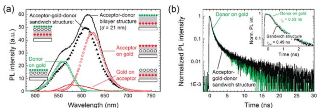
Figure 10 Enhancement of the NRET in the CdTe QD–Au nanoparticle layer-by-layer coated system investigated using (a) steady-state and (b) time-resolved spectroscopy. (a) Using four different negative control samples (donor on gold, acceptor on gold, gold on acceptor and acceptor–donor bilayer structure) and the working sample (acceptor–gold–donor sandwich structure) steady-state emission properties of the QDs were compared. (b) In the time-resolved decay curves, modification of the exciton lifetime of the donor QDs at a large separation distance was shown in the presence and absence of the gold nanoparticles. The acceptor–gold–donor structure exhibits faster donor lifetime as compared to the case of donor on gold, which is attributed to the enhanced NRET due to the gold nanoparticles. [Reprinted (adapted) with permission from ref. [219] (Copyright 2011 American Chemical Society).]
