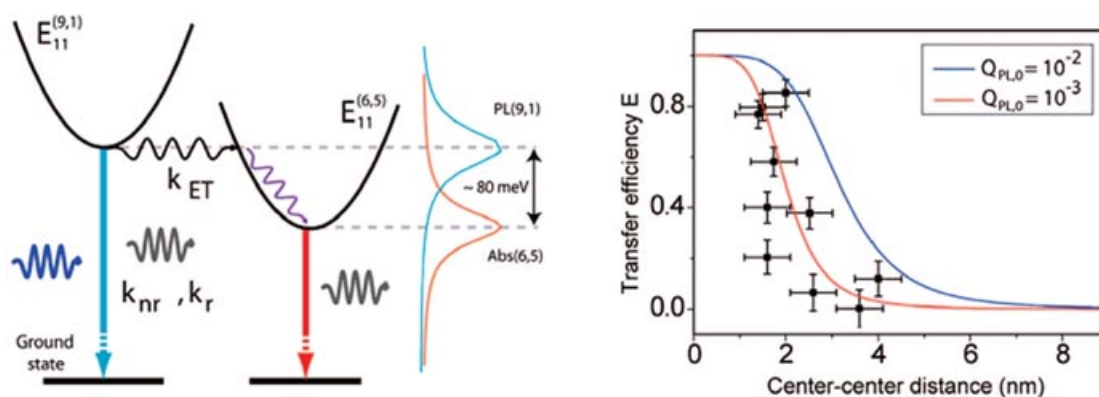
Figure 8 Exciton transfer via NRET in the SWCNT bundles. Similar to NRET in QD assemblies, NRET can occur in the CNT bundle from a larger-bandgap CNT to a smaller-bandgap CNT. Energy-transfer efficiency was plotted as a function of separation distance between the two interacting CNT for the two cases of PL QY. For the separation distance NRET becomes efficient. [Reprinted (adapted) with permission from ref. [200] (Copyright 2008 American Chemical Society).]
