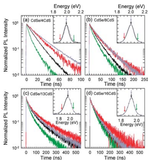
Figure 1 Time-resolved fluorescence decay measurements of the CdSe/CdS QDs depicted with respect to different CdS shell thicknesses (i.e. 4, 8, 13 and 16 monolayers). Decay measurements are performed for one QD distribution having only inhomogeneous broadening due to finite size distribution. Measurements were performed at three different spectral positions of the QD emission (i.e. higher- and lower-energy tails and at the peak) in thin film (green, black and red curves), and also at the peak position in the solution phase of the same QDs (gray curve). As the shell thickness is increased, NRET process is suggested to be suppressed in the solid-state films of the QDs because the decay curves at different positions of the QD emission spectrum become similar. Furthermore, as the shell thickness increases, the thin film and solution phase decay curves for the peak position become almost the same, which indicates the isolation of the emitting cores of the QDs due to the thick shells. [Reprinted (adapted) with permission from ref. [67] (Copyright 2012 American Chemical Society).]
