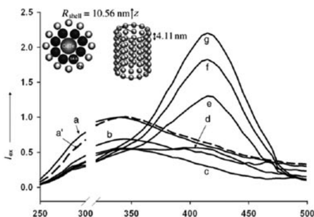
Figure 9 Schematics of the CdTe–Ag nanowire–nanocrystal structure with enhanced emission properties due to the photon–plasmon resonance. The structure was assembled in a solution using special biolinkers (SA–B). The plot shows the photoluminescence excitation (PLE) spectra at the peak emission wavelength of the CdTe nanocrystals. After every 10 min, PLE spectrum is measured for (a)–(g). As the CdTe–Ag hybrid is formed in solution, the significant enhancement in PLE signal is observed at \sim 420 nm. The schematic shows a cross section with a central CdTe NW and an Ag-nanoparticle shell. Reprinted by permission from Wiley (ref. [216]), Copyright © 2006 Wiley-VCH Verlag GmbH & Co. KGaA, Weinheim
