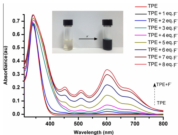
Figure 1. Absorbance spectra of compound 5 + \text{F}^- in the presence of increasing \text{F}^- concentrations. The inset is a digital photograph of the probe (left) and probe following the addition of 8 equivalents of \text{F}^- (right). Probe concentration is 50 \mu\text{M} in DMF.
