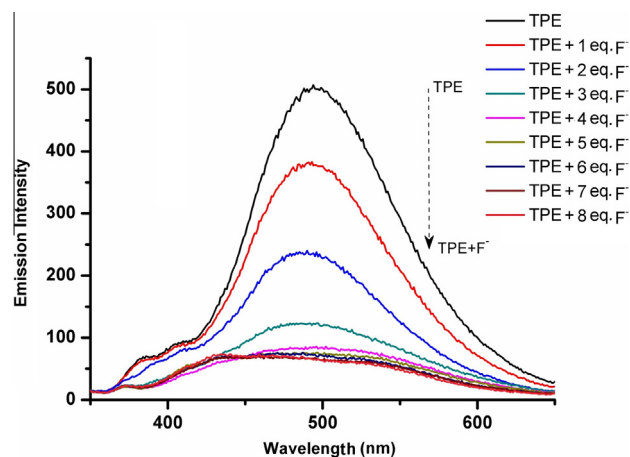
Figure 3. Emission spectra of compound 5 + \text{F}^- in the presence of increasing \text{F}^- concentrations. Probe concentration is 50 \mu\text{M} in DMF. Excitation wavelength is 340 \text{ nm} .
