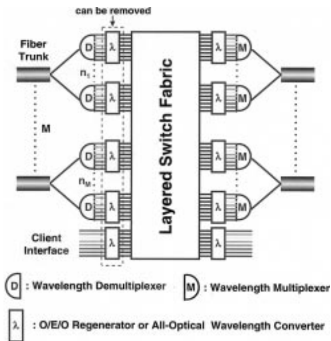
Fig. 1. The switch fabric in each network node can utilize the O/E/O regenerators or all optical wavelength converters to eliminate the wavelength dependence.
