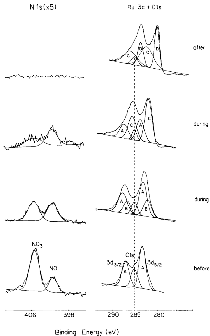
Fig. 2. N 1s and Ru 3d regions of the XPS spectra of Ru(NO)(NO 3 ) 3 , before, during and after annealing up to 170°C in the UHV chamber of the spectrometer. A, B, C and D refer to the +4, +3, +2 and 0 oxidation states of Ru respectively.
