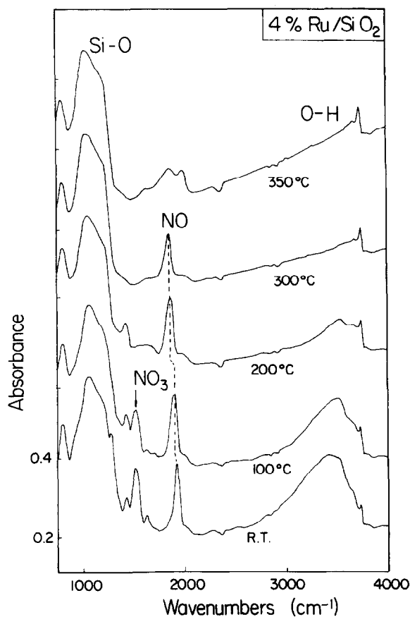
Fig. 1. Mid-IR diffuse-reflectance spectra of 4% Ru catalyst precursor dispersed in silica and after reduction in hydrogen for 1 h at the indicated temperatures.
